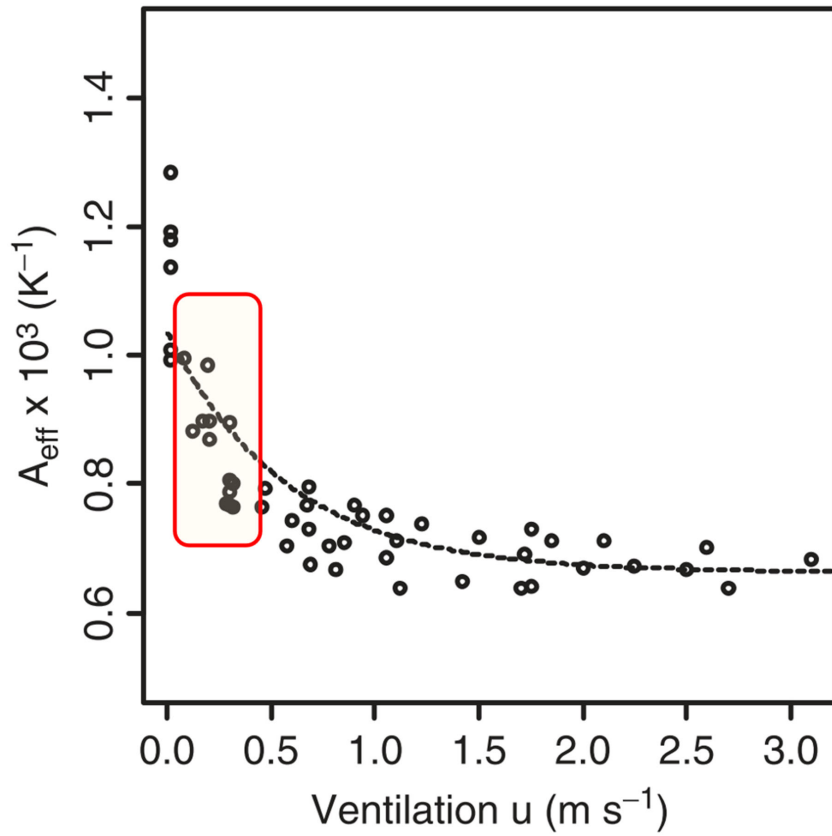
675 Figure 11. Dependence of psychrometer coefficient A on ventilation speed. From Harrison (2014), Figure 6.18. Shaded box overlay shows the 5 and 95 percentile limits of screen airflow observed during this experiment.
