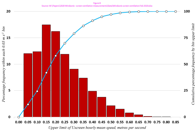
665 Figure 8. Percentage frequency distribution of hourly mean screen ventilation U_{\text{screen}} within 0.05 \text{ m s}^{-1} bins. Red columns show per-bin frequency (left vertical axis), blue line and markers cumulative percentage frequency below upper bin limit (right vertical axis). Total 2423 observations, hourly mean speed 0.20 \text{ m s}^{-1} , median 0.18 \text{ m s}^{-1} , minimum 0.01 \text{ m s}^{-1} , maximum 0.78 \text{ m s}^{-1} .
