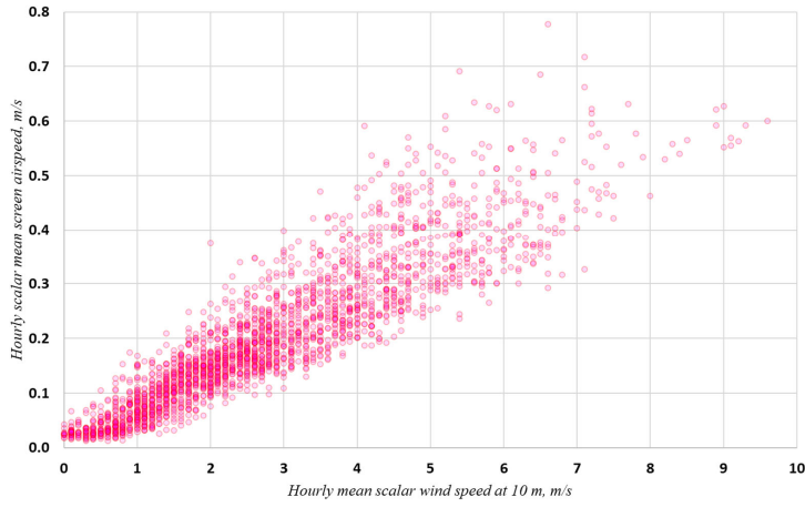
200 Fig. 3. Hourly scalar mean wind speeds within the screen ( U_{screen} ) plotted against the external 10 m scalar mean wind speed U_{10} , for the period 13 February to 27 May 2020. Units m\ s^{-1} .
