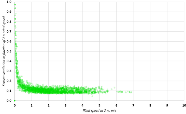
205 Fig. 5. As Fig. 4, but for U_2 , based on hourly scalar means. A few values of U_{screen} > U_2 are omitted for clarity—see text. Above about 1 \text{ m s}^{-1} U_{screen} ventilation averaged about 10% of U_2 .
