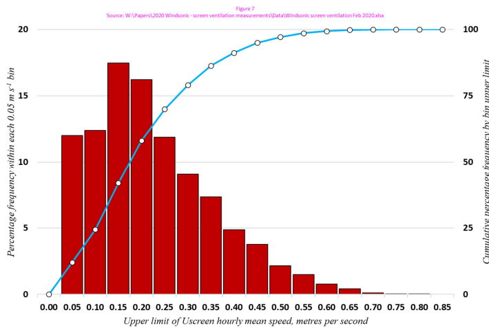
Fig. 7. Percentage frequency distribution of hourly mean screen ventilation U_{screen} within 0.05 \text{ m s}^{-1} bins. Red columns show per bin frequency (left vertical axis), blue line and markers cumulative percentage frequency below upper bin limit (right vertical axis). Total 2423 observations, hourly mean speed 0.20 \text{ m s}^{-1} , median 0.18 \text{ m s}^{-1} , minimum 0.01 \text{ m s}^{-1} , maximum 0.78 \text{ m s}^{-1} .
