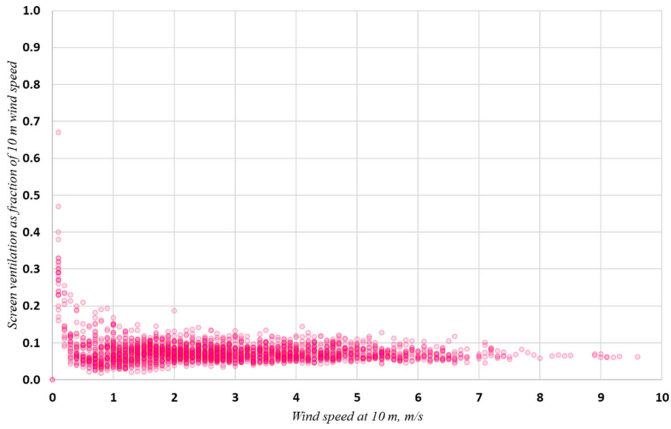
655 Figure 5. Scatterplot of U_{\text{screen}} as a fraction of U_{10} , based on hourly scalar means. Above about 1 \text{ m s}^{-1} U_{\text{screen}} \approx 7\% of U_{10}
