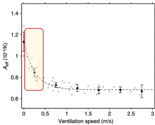
435 Fig. 10. Dependence of psychrometer coefficient A on ventilation speed. From Harrison and Wood (2012), Fig. 3. Shaded box overlay shows the 5 and 95 percentile limits of screen airflow observed during this experiment.
