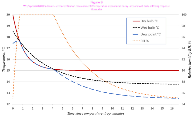
Figure 9. Time series (minutes) of dry-bulb, nominal wet-bulb and calculated dew point temperatures (°C, left axis) and relative humidity (%RH, right axis) following an instantaneous fall in temperature of 5 K from 20 °C, assuming sensor response times per Table 2
