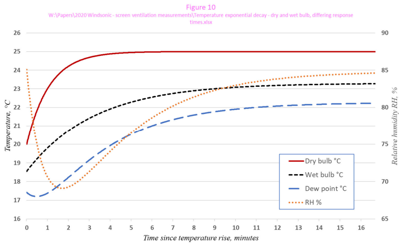
Figure 10. As Figure 9, but for an instantaneous rise in temperature of 5 K from 20 °C
