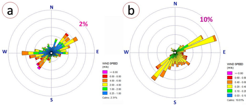
660 Figure 7. Hourly vector mean wind direction frequencies, in wind rose format, during the experimental period: a. at 10 m; b. within the Stevenson screen. Note that the scales and class boundaries necessarily differ - the outer scale ring representing 2% frequency for the 10 m plot and 10% for the screen. Mean wind speed 2.8 \text{ m s}^{-1} at 10 m, 0.20 \text{ m s}^{-1} within the screen.
