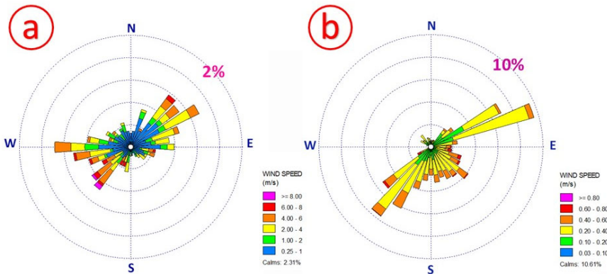
Fig. 6. Hourly vector mean wind direction frequencies, in wind rose format, during the experimental period: a, at 10 m; b, within the Stevenson screen. Note that the scales and class boundaries necessarily differ – the outer scale ring representing 2% frequency for the 10 m plot and 10% for the screen. Mean wind speed 2.8 m s -1 at 10 m, 0.20 m s -1 within the screen.
