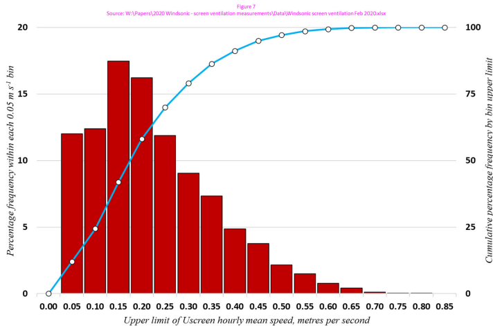
270 Fig. 7. Percentage frequency distribution of hourly mean screen ventilation U_{screen} within 0.05 \text{ m s}^{-1} bins. Red columns show per-bin frequency (left vertical axis), blue line and markers cumulative percentage frequency below upper bin limit (right vertical axis). Total 2423 observations, hourly mean speed 0.20 \text{ m s}^{-1} , median 0.18 \text{ m s}^{-1} , minimum 0.01 \text{ m s}^{-1} , maximum 0.78 \text{ m s}^{-1} .
