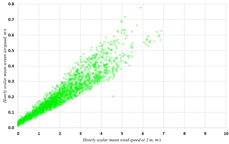
Figure 4. As Figure 3, but for 2 m scalar mean wind speed U_2 .
