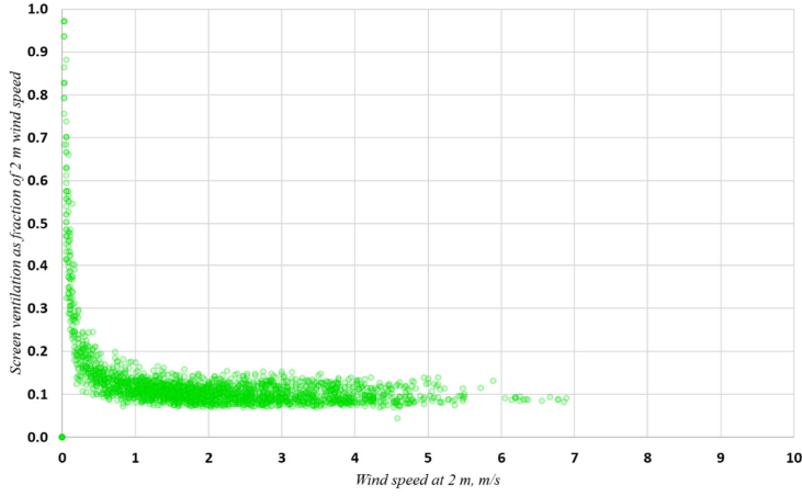
Fig. 5. As Fig. 4, but for U_2 , based on hourly scalar means. A few values of U_{screen} > U_2 are omitted for clarity—see text. Above about 1 \text{ m s}^{-1} U_{screen} ventilation averaged about 10% of U_2 .
