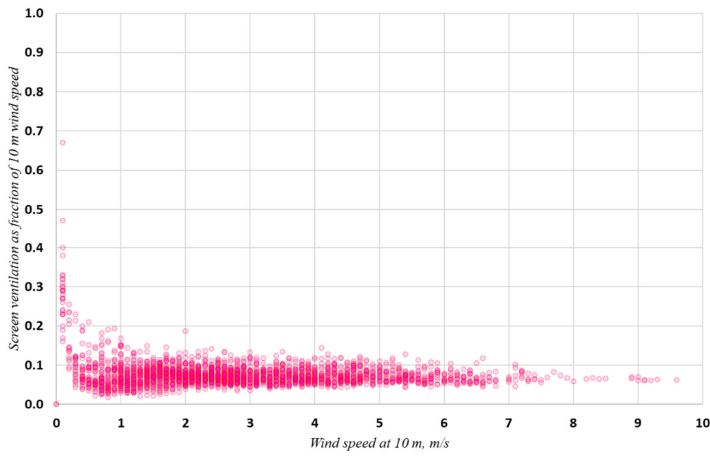
Figure 4 - Uscrn scalar fraction U10m
