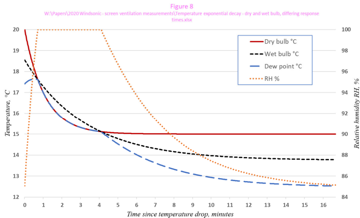
Fig. 8. Time-series (minutes) of dry-bulb, nominal wet-bulb and calculated dew-point temperatures (°C, left axis) and relative humidity (RH %, right axis) following an instantaneous fall in temperature of 5 K from 20 °C, assuming sensor response times per Table 2
