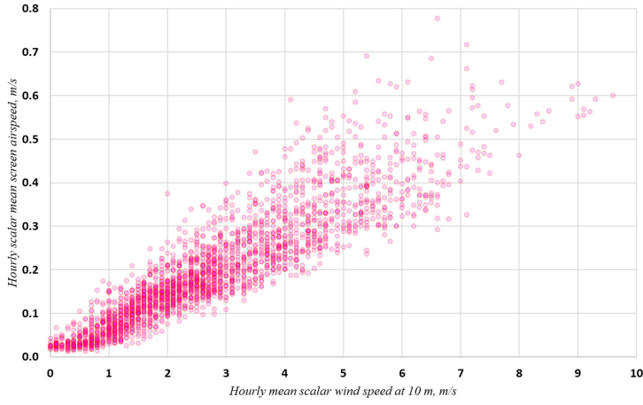
Fig. 3. Hourly scalar mean wind speeds within the screen ( U_{scrn} ) plotted against the external 10-m scalar mean wind speed U_{10} , for the period 13 February to 27 May 2020. Units m s^{-1} .
