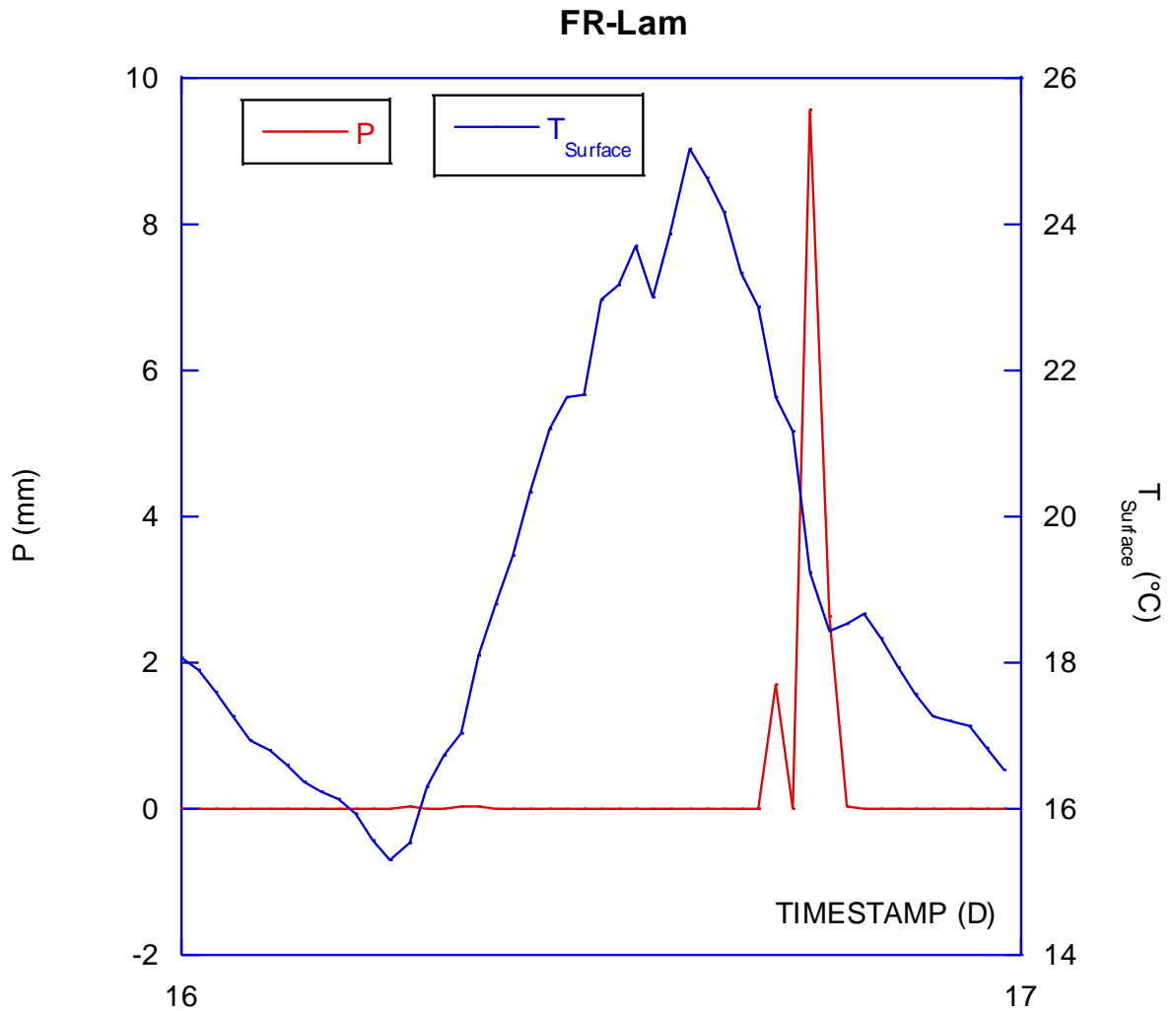
305 Figure 6. Rainfall soil surface temperature cooling.
