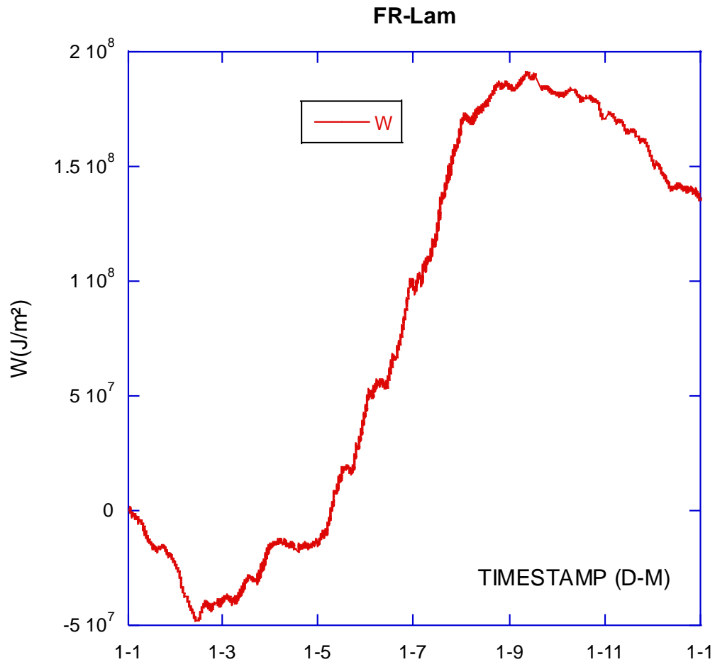
Figure 2. Soil heat flux Integrated during for one year.
