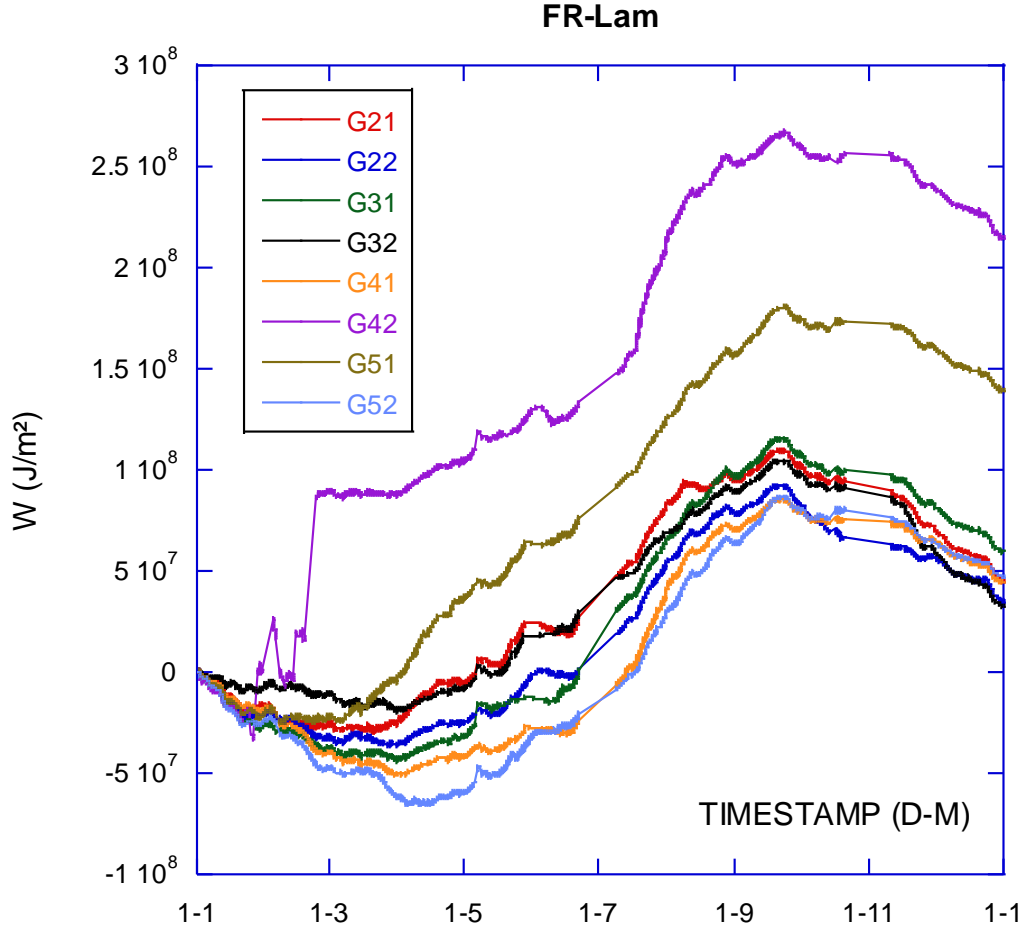
260 Figure 4. Integrated raw measurements of eight heat flux plates installed on FR-Lam on an agricultural plot (cropland).
