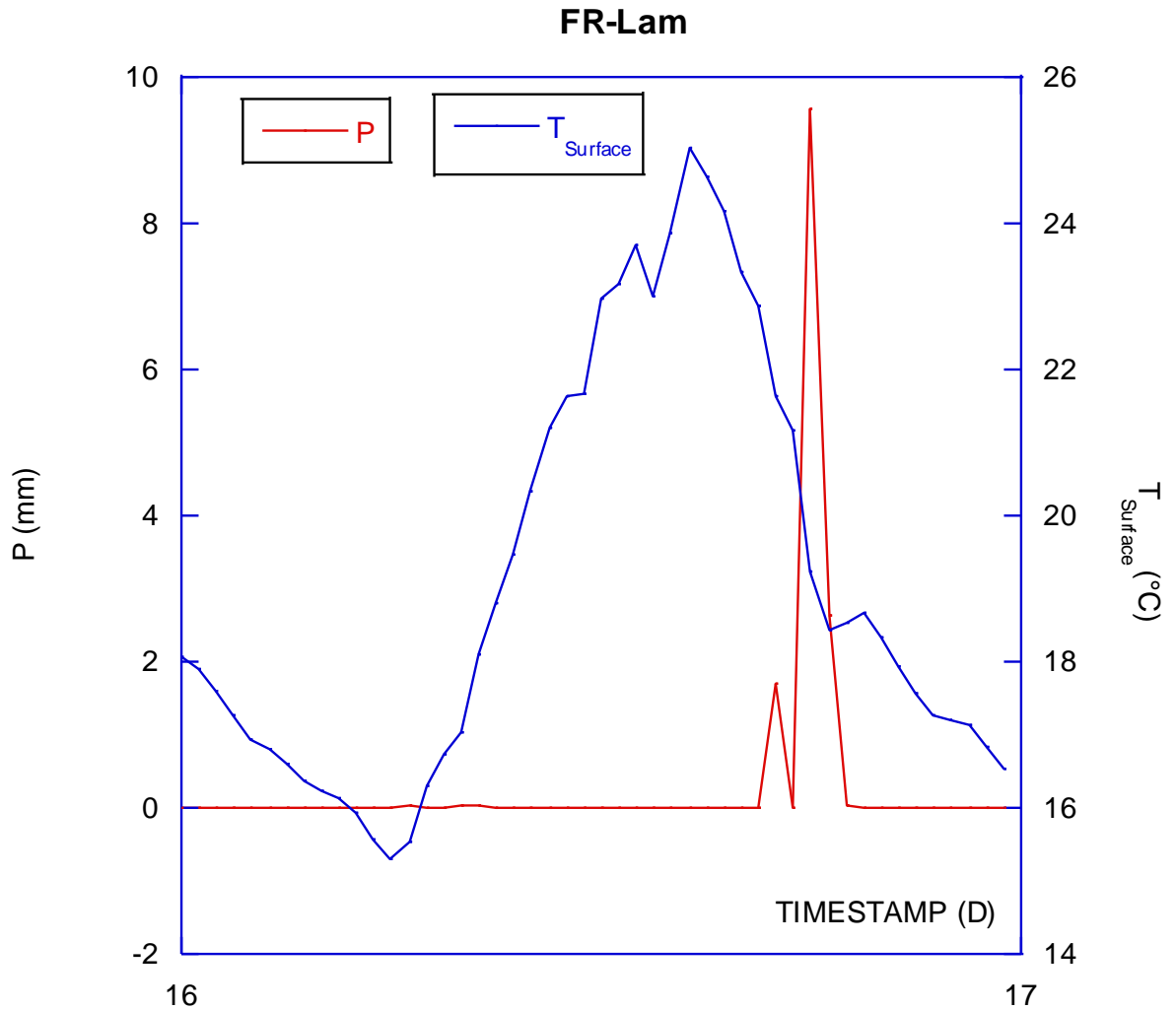
300 Figure 6. Rainfall soil surface temperature cooling.
