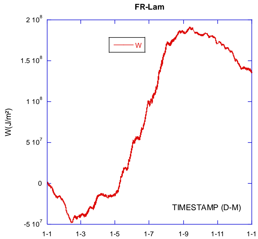
Figure 2. Soil heat flux Integrated for one year.
