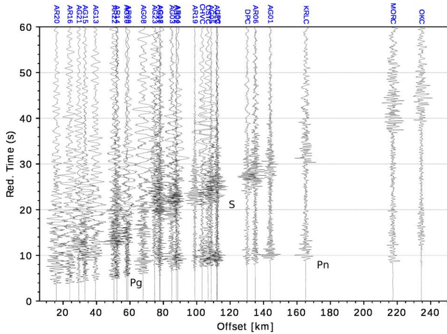
Figure 8. Example of waveforms recorded for the M4.4 local earthquake which occurred 2018-07-03, 19:38:47.75 UTC in Legnica-Głogów Copper District (lat: 51.5145, lon: 16.1378, depth: 0.0 km after ISC). Band-pass filter 0.2-15 Hz was used. Reduction velocity is 8 km/s. Location of the epicenter is shown in Figure 2.
