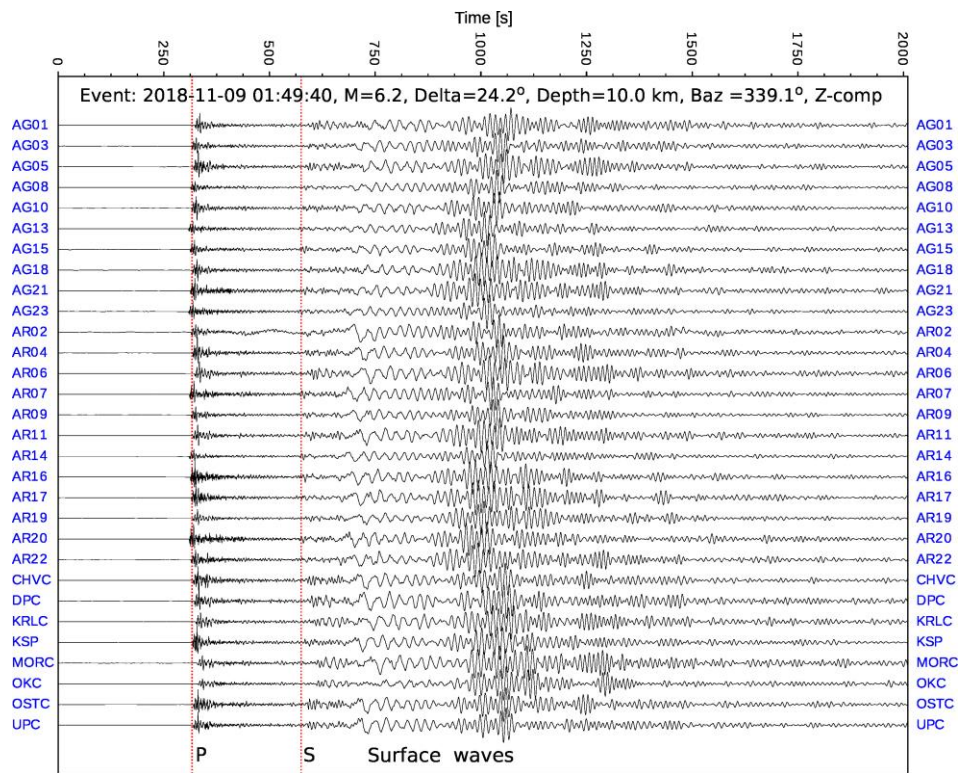
265 Figure 6: Example of vertical component of recorded waveforms for the M6.2 teleseismic earthquake which occurred 2018-11-09 in Jan Mayen Island region (lat: 71.6312, lon: -11.2431, depth: 10.0 km after ISC). Red lines mark the theoretical onsets of P- and S-phases at the KSP station. All seismograms are low-pass filtered (< 1 Hz).
