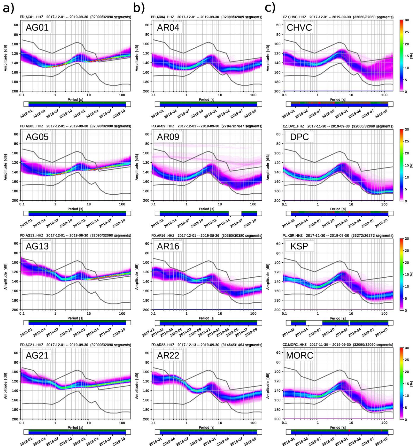
335 Figure 12: Probabilistic power spectral density (PPSD) on the Z-component for 12 selected stations. a) CMG-6T sensors, b) RT 151-120 sensors, c) permanent stations. Black lines mark New High and Low Noise Models (NHNM, NLNM; Peterson 1993).
