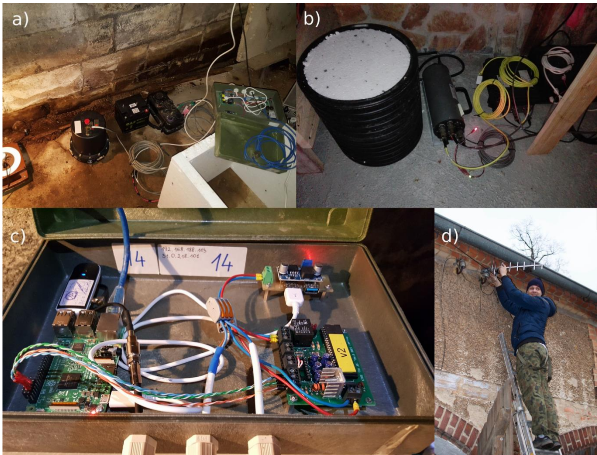
Figure 3: Deployment of seismic stations in the Sudetes: a) Reftek unit during installation, b) Installed Güralp unit, c) data-transmission module – Raspberry Pi microcomputer with UMTS modem and watchdog, d) Installing the UMTS antenna for data transmission.
