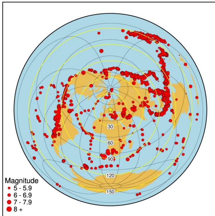
260 Figure 4: Distribution of the epicenters of M > 5.5 earthquakes in the period from 18 Oct 2017 to 26 Oct 2019, according to ISC catalogue (1285 events). The yellow asterisk represents the center of the AniMaLS seismic array in the Sudetes. The yellow circles mark the distances (in degrees) from the array center in 30^\circ steps.
