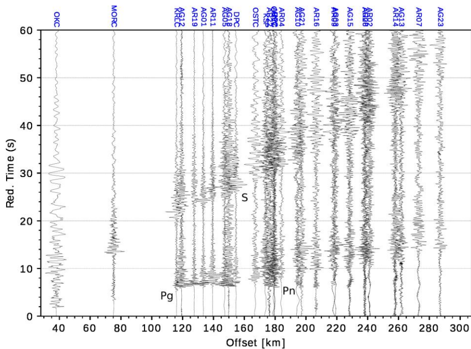
Figure 9: Example of waveforms recorded for the M3.9 local earthquake which occurred 2019-01-22, 22:35:30.08 UTC in Upper Silesia district (lat: 50.1095, lon: 18.4559, depth: 5.5 km after ISC). Band-pass filter 0.2-15 Hz was used. Reduction velocity is 8 km/s.
