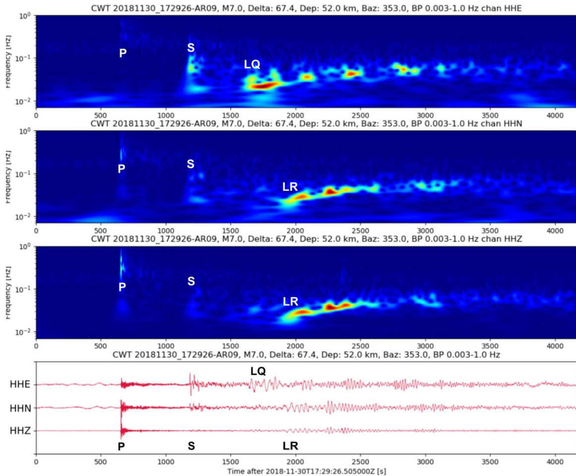
Figure 10: Spectral seismograms obtained with the use of continuous wavelet transform for station AR09, showing a teleseismic event from Southern Alaska, 2018-11-30, 17:29:26 UTC. From top to bottom: E-, N- and Z-component.
