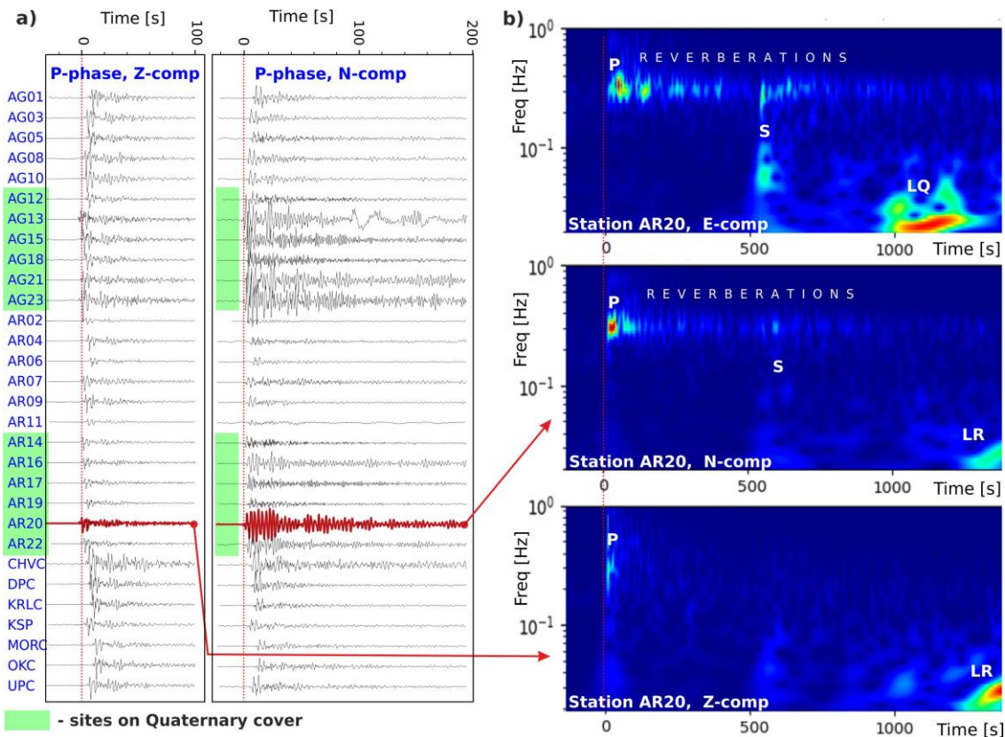
Figure 14: Seismic data example for event from 2018-11-30, 17:29:26 UTC, illustrating the differences in P-phase records between stations located on consolidated basement (short pulse, no reverberations) and sites located on young, unconsolidated cover (green rectangles, strong reverberations on the horizontal components). a) Z- and N-component records for all the stations used. b) 3-component spectral seismograms for station AR20. E- and N-components show high amplitude, > 600 s long coda (reverberations) in a narrow frequency range, centered at 0.3 Hz. The coda is non-existent in the Z-component record. True amplitude scaling was applied. Time scale is relative to theoretical P-phase onset.
