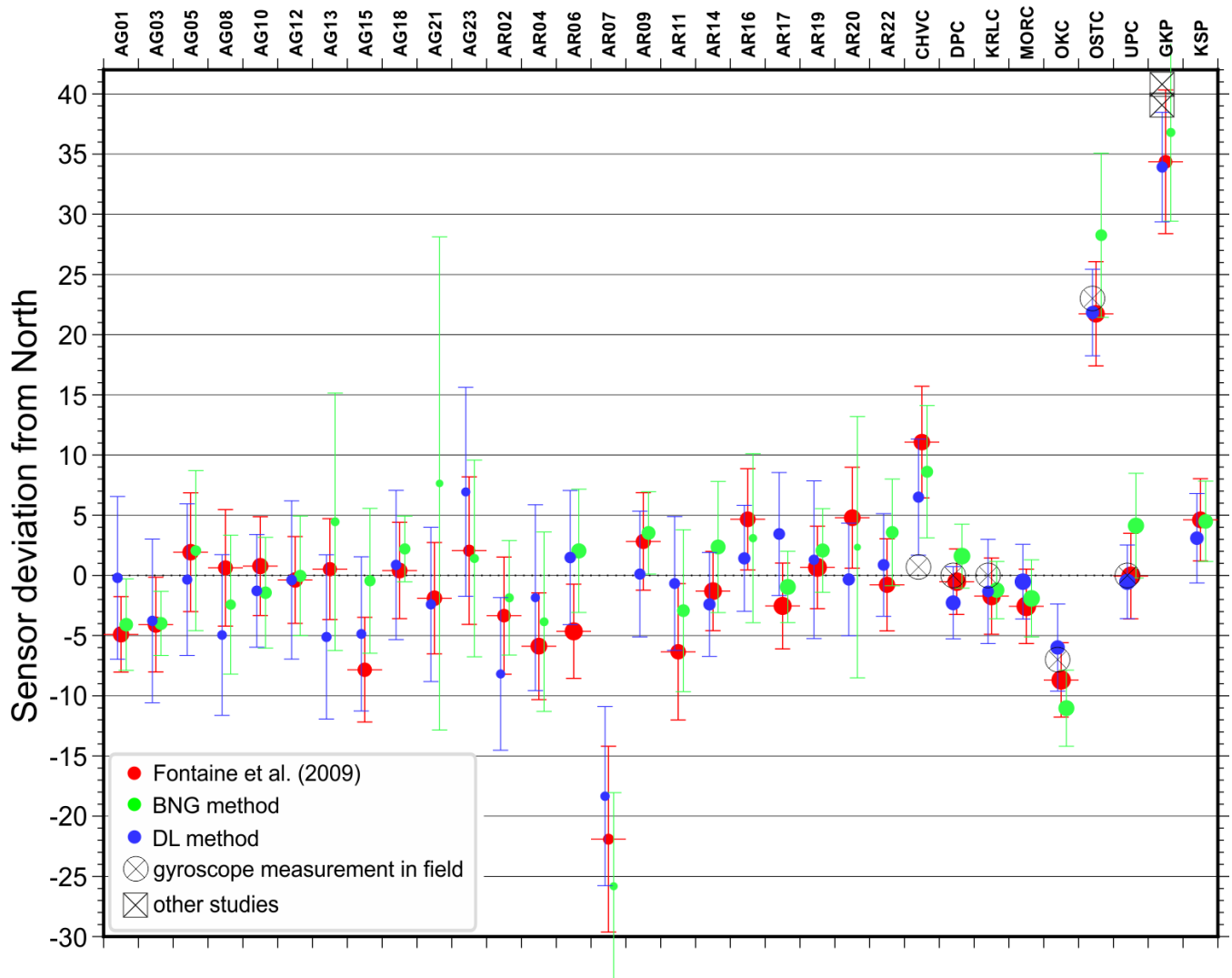
450 Figure 15: Misorientation angles calculated for all stations using three described methods: red dots – Fontaine et al. (2009) method, green dots – BNG method, blue dots – DL method. Black circles with crosses – orientation angles of permanent stations from direct, high accuracy measurements in field by gyrocompass (Vecsey L., Institute of Geophysics of Czech Academy of Sciences, personal communication, 2020). Black squares with crosses (for GKP station) – orientation angles reported by other studies (Vecsey et al., 2014; Wilde-Piórko et al., 2017).
