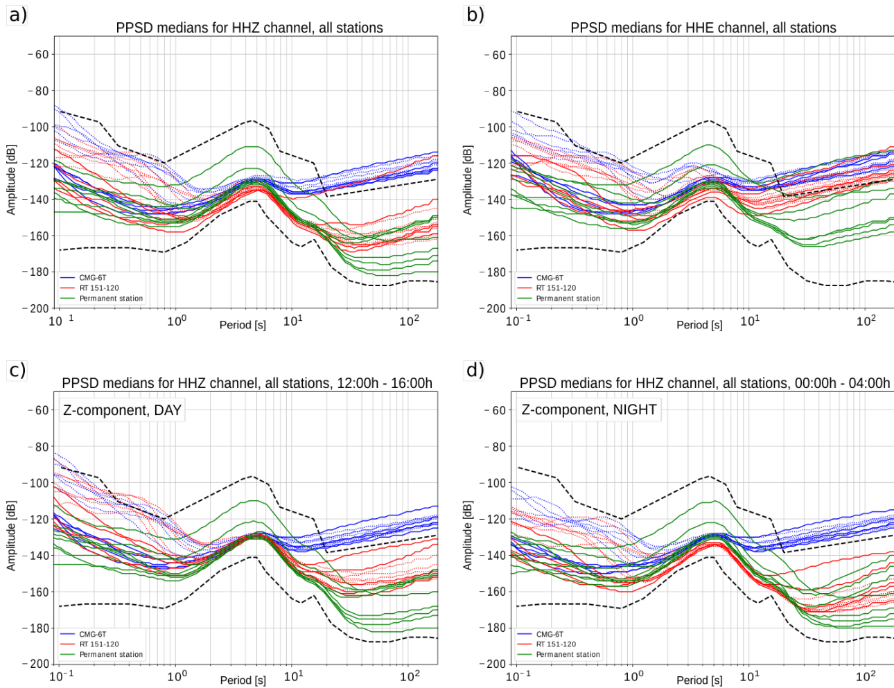
Figure 13: The PPSD median curves for all temporary and permanent stations. a) Z-component, b) E-component, c) Z-component, day hours only (12:00-16:00 local time), d) Z-component, night hours only (00:00-04:00 local time). Dotted lines – stations located on Quaternary sediments, solid lines - stations located on Palaeozoic or older basement. Time span for calculation is 22 months from Jan 2018 to Oct 2019. Black lines mark New High and Low Noise Models (NHNM, NLNM; Peterson 1993).
