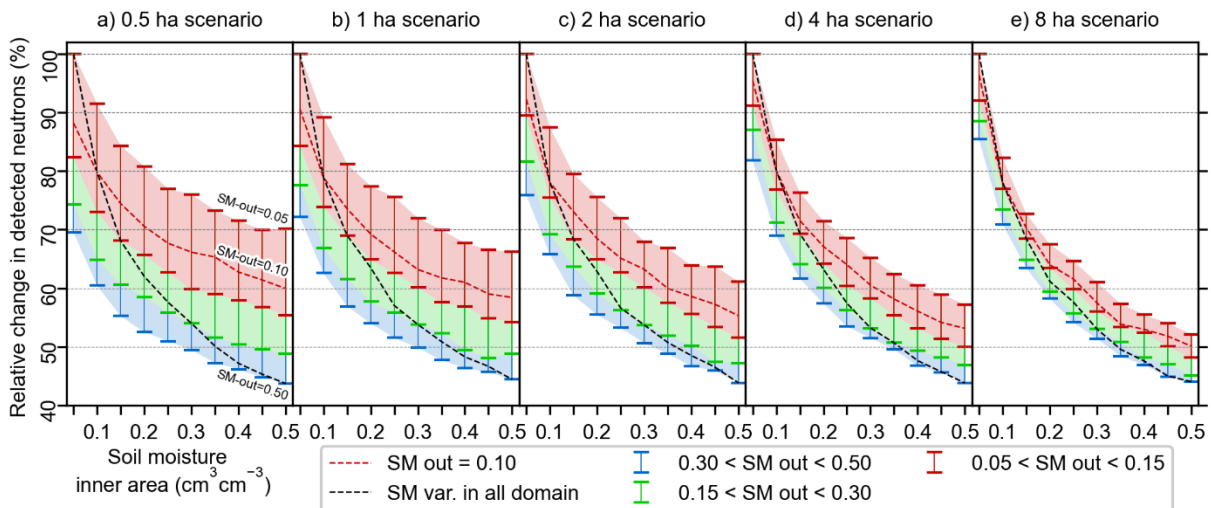
395 Figure 9: Relative changes in detected neutrons due to SM variations in a) 0.5 ha, b) 1 ha, c) 2 ha, d) 4 ha, and e) 8 ha irrigated areas. The black dashed line shows SM variations that are homogeneous within the simulated domain. The red dashed lines and the error bars indicate SM variations that occur only within the irrigated area for a different SM in the outer area.
