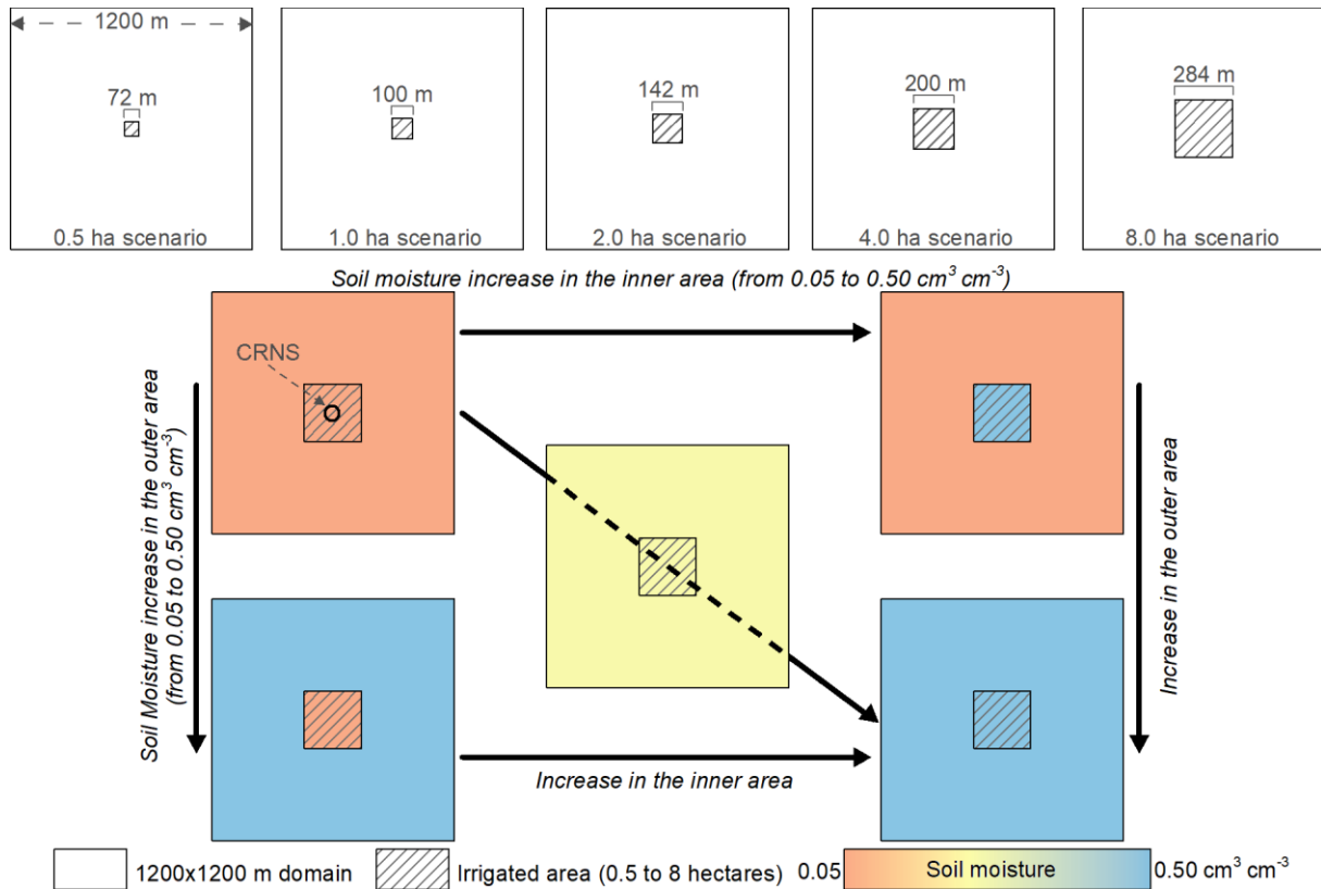
170 Figure 1: Examples of the dimensions of the inner area relative to the simulation domain and schematization of the simulation design and setup with an example for the 8 ha scenario. A 1200x1200 m domain is used with an inner area of 8 ha and a CRNS placed at its centre. The SM is then systematically varied in the inner and outer area with increments of 0.05 \text{ cm}^3 \text{ cm}^{-3} for a total of 100 simulations.
