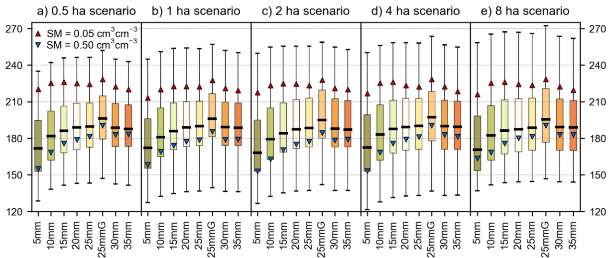
255 Figure 3: Boxplots of R86 in meters for different moderator types and size of the inner area, i.e. a) 0.5 ha, b) 1 ha, c) 2 ha, d) 4 ha, and e) 8 ha. Each boxplot refers to one moderator type (100 combinations of SM) and shows the minimum and maximum values with whisker caps, the interquartile range with bars, and the median with a black line. Blue and red triangles show R86 values for homogeneous SM of 0.05 and 0.50 cm 3 cm -3 respectively.
