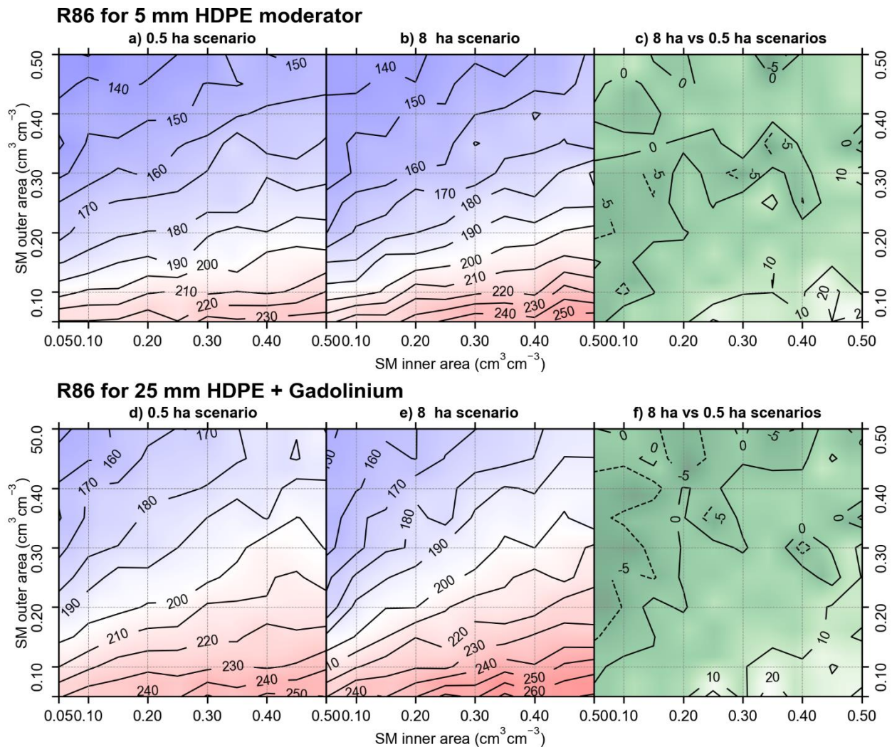
280 Figure 4: Variation of R86 with SM using a 5 mm HDPE moderator for the a) 0.5 ha and b) 8 ha scenario and using a 25 mm HDPE moderator with gadolinium shielding for d) 0.5 ha and e) 8 ha scenario. The differences between the 8 ha and 0.5 ha scenarios are shown in c) for the 5 mm HDPE moderator and in f) for the 25 mm HDPE moderator with gadolinium shielding. Here, negative values indicate that the footprint of the 8 ha scenario is smaller than that of the 0.5 ha and vice versa.
