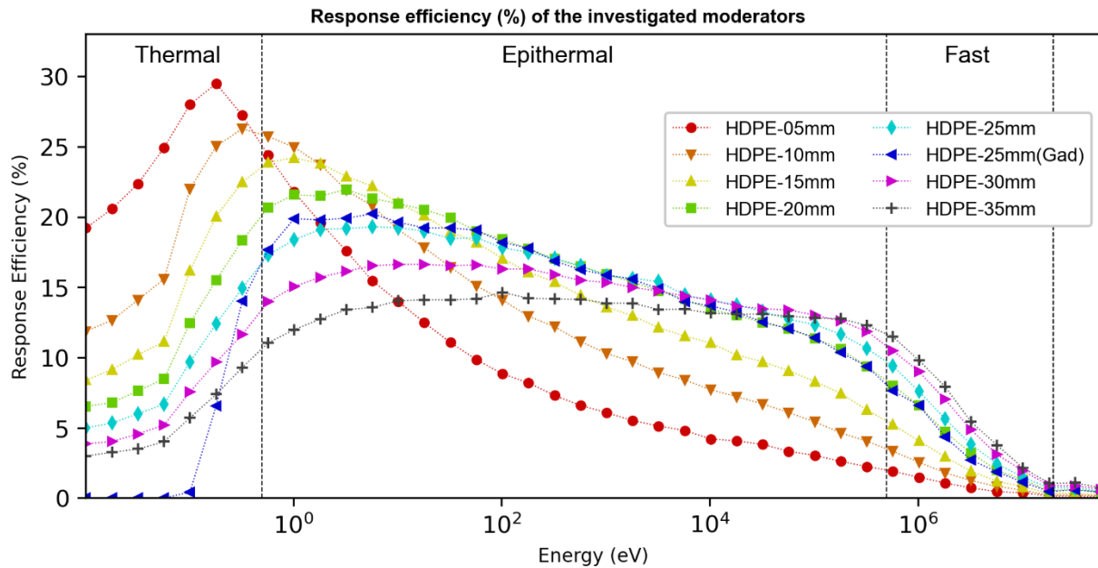
200 Figure 2: Energy dependent response functions of different moderators made of 5 to 35 mm thick high-density polyethylene (HDPE) and, in the case of 25mm HDPE, an additional gadolinium based thermal shielding.
