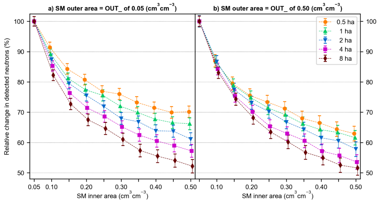
350 Figure 7: Relative change in number of detected neutrons using a 25 mm HDPE moderator with gadolinium shielding for different dimensions of the irrigated area and two different SM in the outer area: a) 0.05 \text{ cm}^3 \text{ cm}^{-3} and b) 0.50 \text{ cm}^3 \text{ cm}^{-3} . The error bars indicate the relative error of the simulations.
