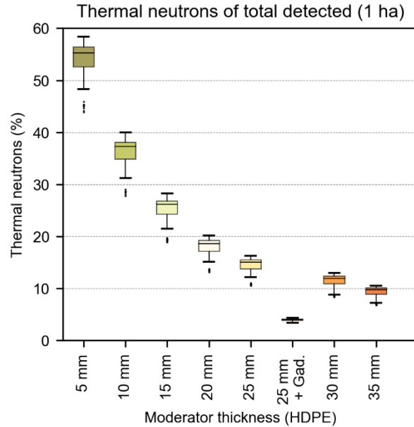
495 Figure B 1: Boxplot of the percentage of detected thermal neutrons over the total number of neutrons that are detected with different moderator types for the 1 ha scenario (each boxplot shows the results of 100 simulations).
