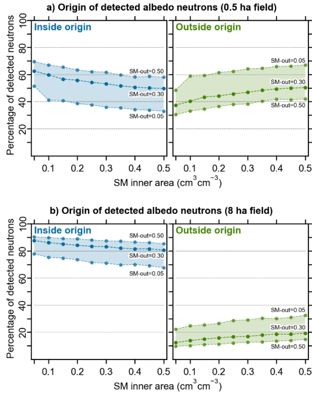
315 Figure 5: Percentages of detected neutrons that originate in the inner and outer area for a) the 0.5 ha scenario and b) the 8 ha scenario. These results are shown for a detector with a 25 mm HDPE moderator with gadolinium shielding.
