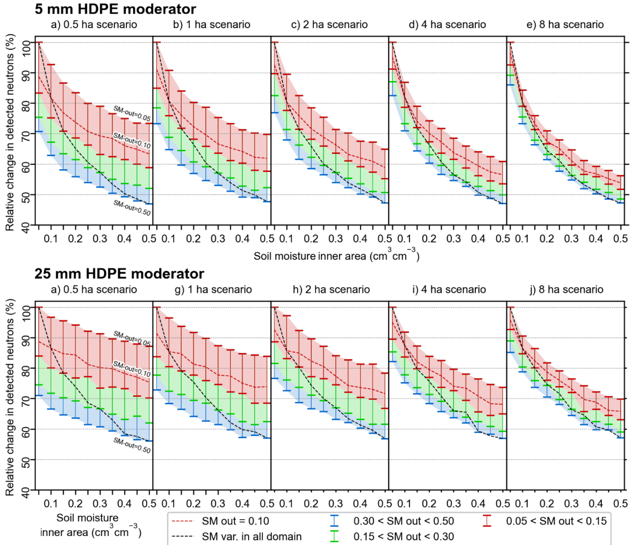
Figure C 1: Relative changes in detected neutrons due to SM variations in a) 0.5 ha, b) 1 ha, c) 2 ha, d) 4 ha, and e) 8 ha irrigated areas for a 5 mm HDPE moderator and in f) 0.5 ha, g) 1 ha, h) 2 ha, i) 4 ha, and l) 8 ha for a 25 mm HDPE moderator. The black dashed line shows SM variations that are homogeneous within the simulated domain. The red dashed lines and the error bars indicate SM variations that occur only within the irrigated area for a different SM in the outer area.
