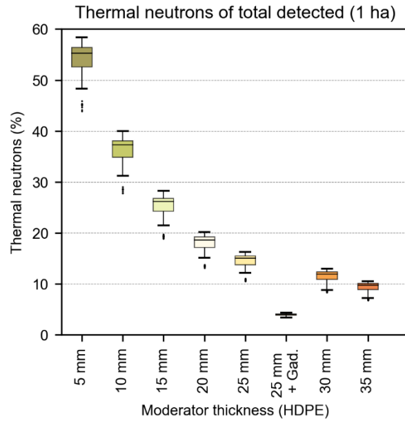
525 Figure B 1: Boxplot of the percentage of detected thermal neutrons over the total number of neutrons that are detected with different moderator types for the 1 ha scenario (each boxplot shows the results of 100 simulations).
