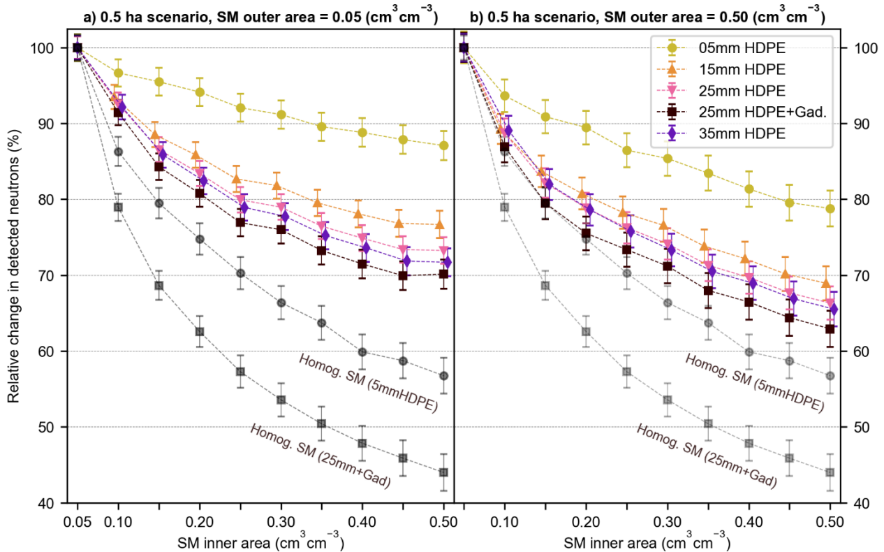
340 Figure 6: Relative change in number of detected neutrons due to SM variations obtained using different moderators (i.e., 5, 15, 25, 35 mm HDPE and 25 mm HDPE with gadolinium shielding) for a) 0.05 \text{ cm}^3 \text{ cm}^{-3} SM and b) 0.50 \text{ cm}^3 \text{ cm}^{-3} SM in the outer area of a 0.5 ha field. The error bars indicate the relative error of the simulations. Grey circles and squares indicate the relative change for two selected moderators when the SM changes from 0.05 to 0.50 \text{ cm}^3 \text{ cm}^{-3} are applied to the entire simulation domain.
