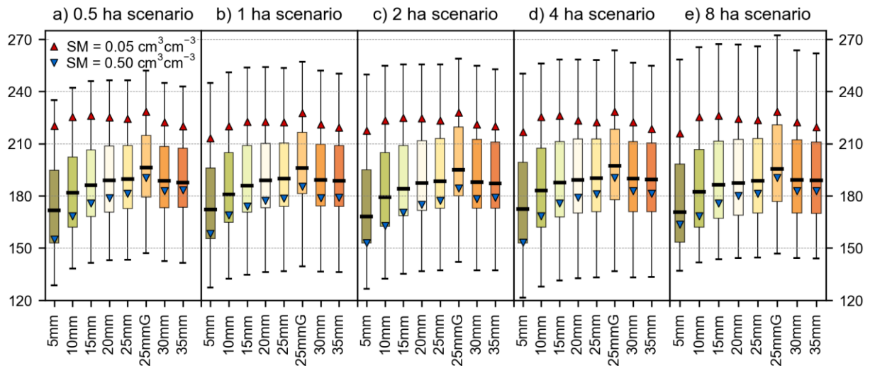
Figure 3: Boxplots of R86 in meters for different moderator types and size of the inner area, i.e. a) 0.5 ha, b) 1 ha, c) 2 ha, d) 4 ha, and e) 8 ha. Each boxplot refers to one moderator type (100 combinations of SM) and shows the minimum and maximum values with whisker caps, the interquartile range with bars, and the median with a black line. Blue and red triangles show R86 values for homogeneous SM of 0.05 and 0.50 \text{cm}^3 \text{cm}^{-3} respectively.
