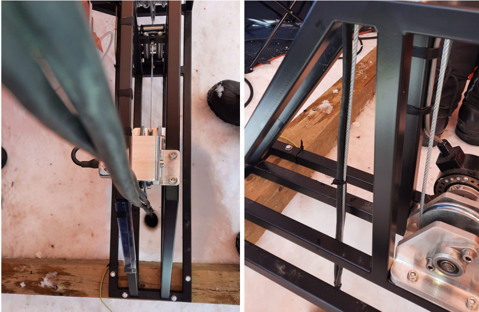
Figure 7 – Overhead (Left) and side (Right) views of the umbilical cable bundled with zip ties prior to entering the borehole.
