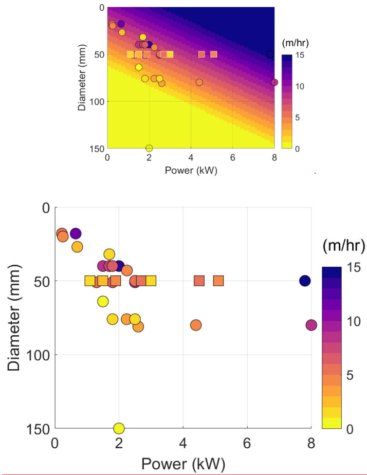
Figure 243 – Rate of penetration as dependent on melt-tip diameter and power. Circles denote previously described melt tip statistics compiled by Talalay [2019]. Background color denotes the expected rate of penetration based on bivariate regression of these previously described melt tip statistics. Squares denote our melt tip performance under both laboratory and field conditions described here.
