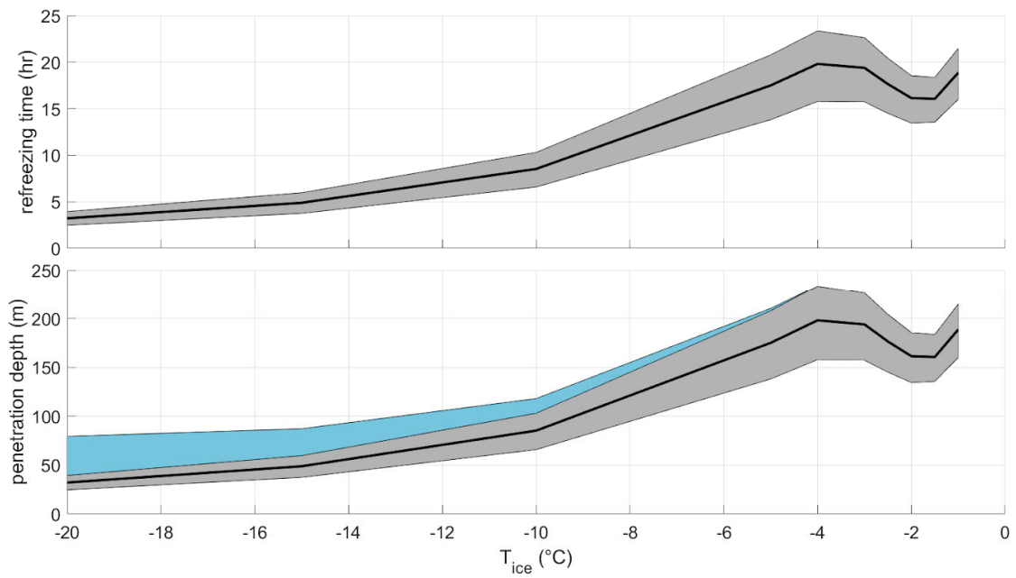
805 Figure 232 – Top: Borehole refreezing time to a characteristic water radius of 1 mm over a variety of ice temperatures. Shaded area denotes 75 \pm 25 °C uncertainty in initial borehole water temperature. Bottom: Maximum theoretical penetration depth of the ice drilling system over a variety of ice temperatures. Grey shaded area corresponds to the shaded area in the top subplot. Blue shaded area reflects the characteristic porous firn depth.
