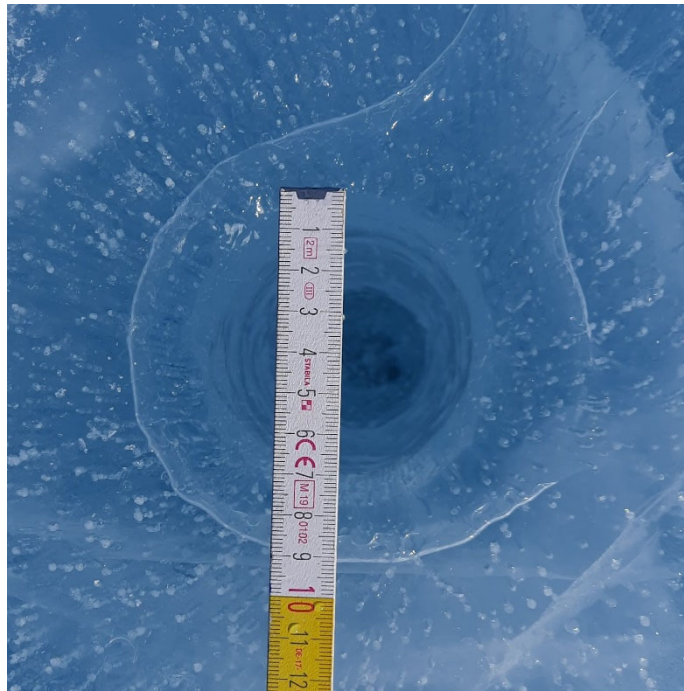
Figure 187 – Testing on the frozen Lake Tuto suggests that the effective borehole diameter of the melt tip is ~70 mm over a wide range of power levels and penetration rates.
