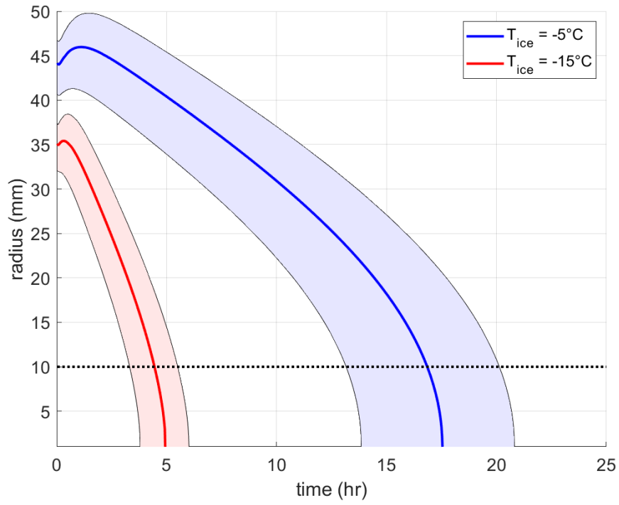
800 Figure 224 – Borehole radius over time solved with a 1-D ice-water moving boundary heat diffusion model. These contrasting simulations depict the differing maximum borehole radii and decay timescales with ice temperatures of -5 and -15 °C. Shaded areas denote 75 \pm 25 °C uncertainty in initial borehole water temperature. Dotted line denotes a 10 mm radius equivalent to the effective cross-sectional area of the umbilical.
