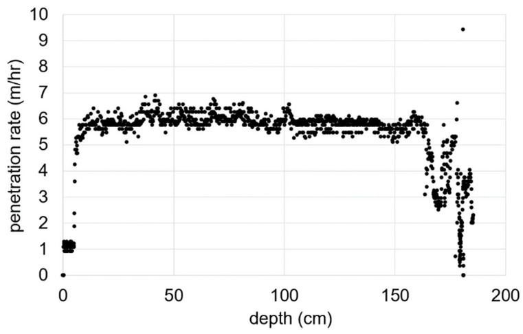
Figure 15 – Rate of penetration measured each second during a 45% power test in the artificial ice well at Jilin University. Aside from initialization and cessation effects, the rate of penetration showed little temporal variance during the steady drilling period ( 5.9 \pm 0.3 m/hr between 25 and 150 cm depth)
