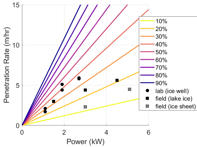
770 Figure 156 – Penetration rate as a function of power for the v2 melt tip in the ice well and the v3 melt tip in the lake ice and ice sheet. For the ice sheet 21 m test, the 1-hour maximum is shown in addition to the test mean. Colored lines indicate heat transfer efficiency in comparison to theoretical perfect heat transfer from the cartridge heaters to melt an ideal borehole.
