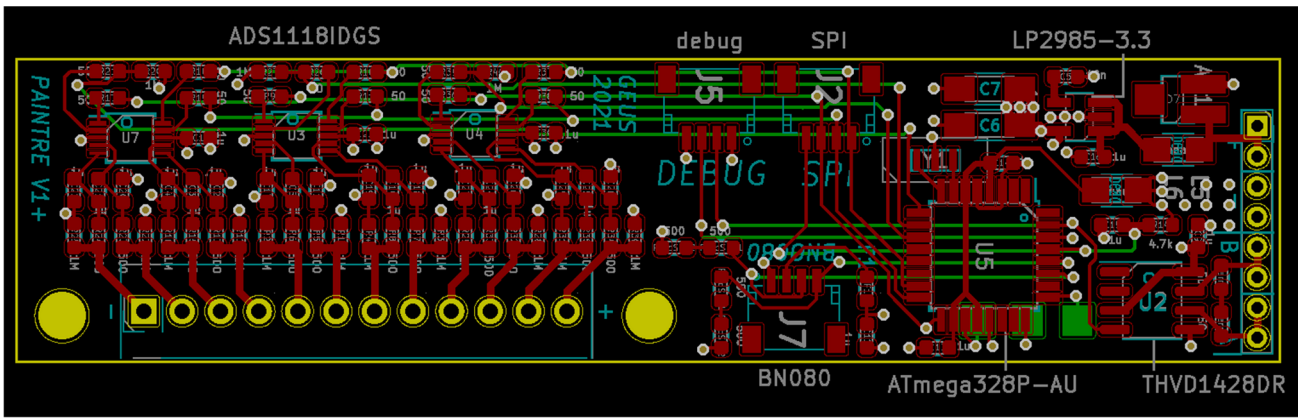
710 Figure 3 – Customized electronics board within the probe that integrates measurements from the cartridge and independent thermocouples as well as the triaxial accelerometer and gyroscope with magnetometer.
