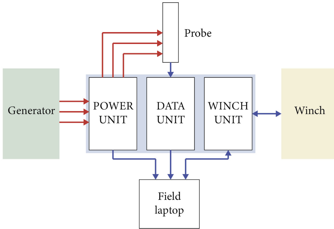
795 Figure 1140 – Diagram of the interface connections to other drilling system components. Red arrows indicate power. Blue arrows indicate data.
