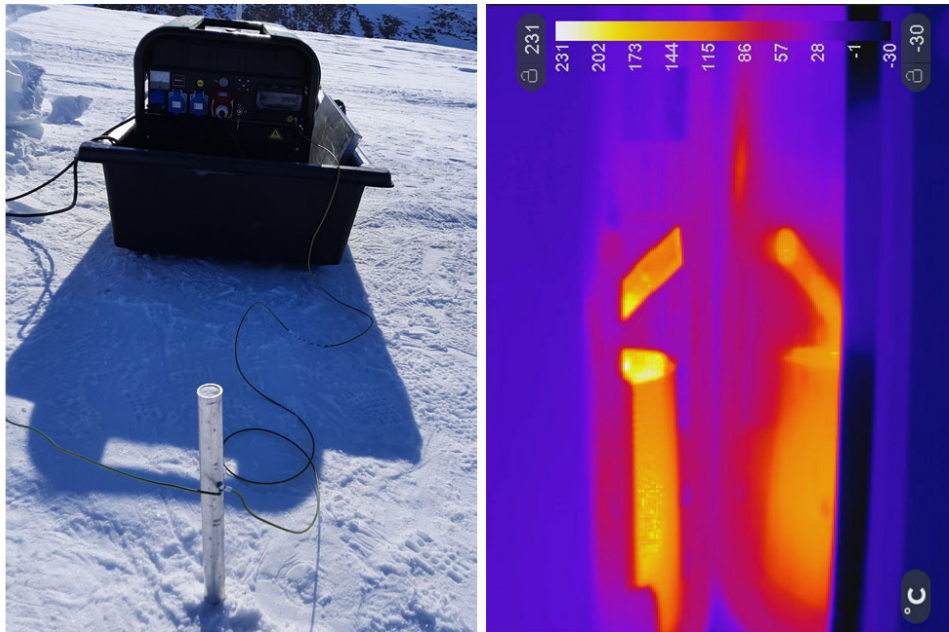
810 Figure 13-14 – Left: Grounding stake drilled into the ice sheet near the generator to ground all electrical elements of the drilling system. Note the metal heat deflector beside the generator, protecting the high-density plastic snowmobile sled. Right: Thermal image of the generator exhaust pipe and its reflection in the metal heat deflector.
