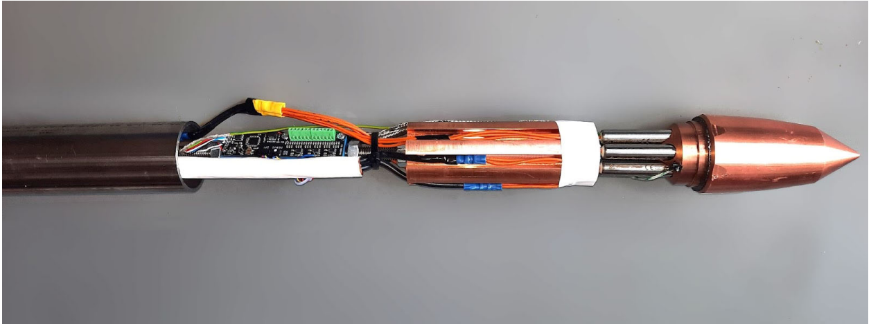
Figure 54 – Overview of the internal construction of the melt tip before resin casting.
