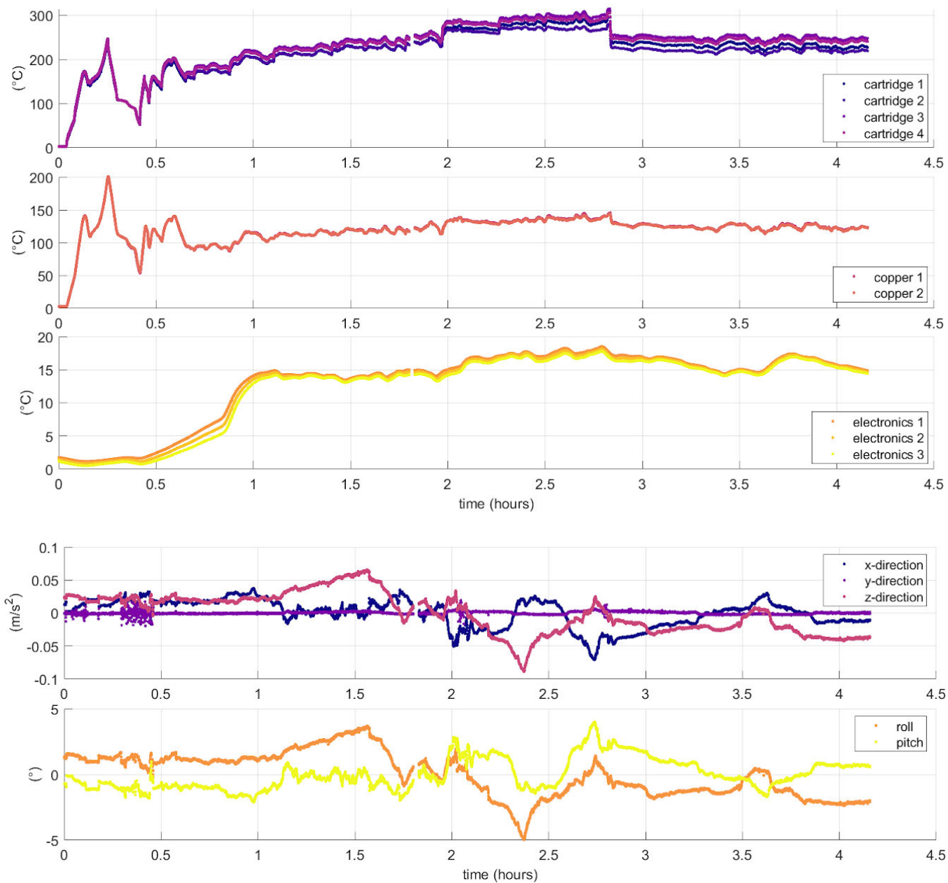
805 Figure 12-13 – Sample of melt-tip data feedback during ice-sheet drilling on 13 May 2022. Top to Bottom: temperatures in four cartridge heaters; temperatures in two spots in the copper heating block; temperature at three places on the electronics board; 3-D acceleration; roll and pitch.
