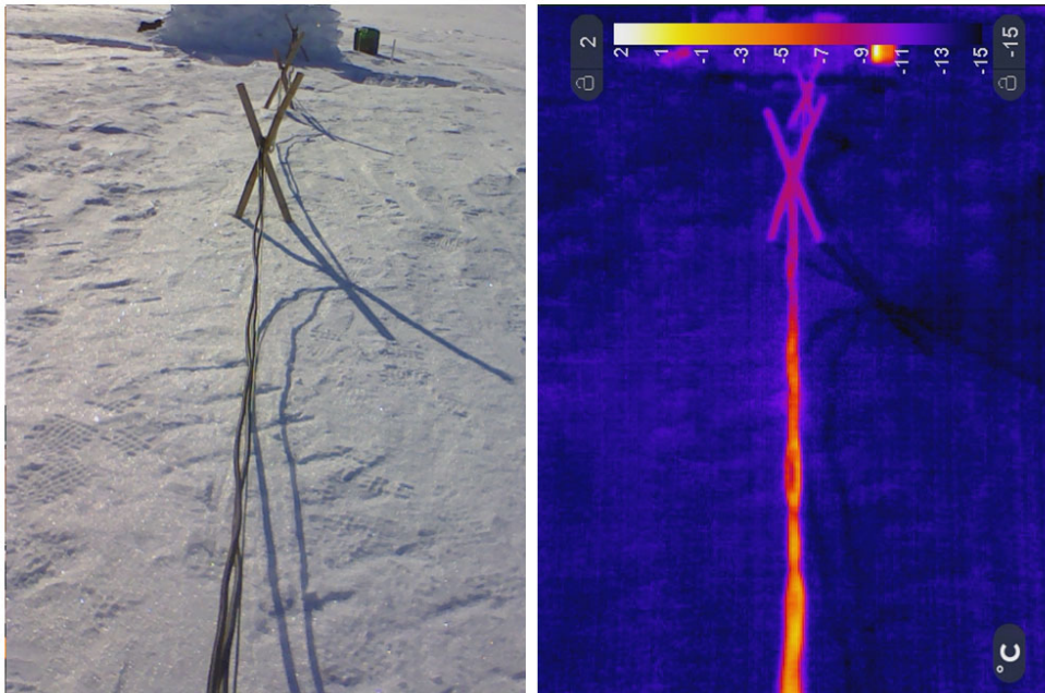
785 Figure 28 – The effect of resistive heating of power cables during field testing. Left: Visible image of the 230 and 400 V power cables from the generator to the drilling tent. Right: Thermal image of the same cables highlights that current flow warms the cable to 0 °C, despite an ambient air temperature of -10 °C with light winds.
