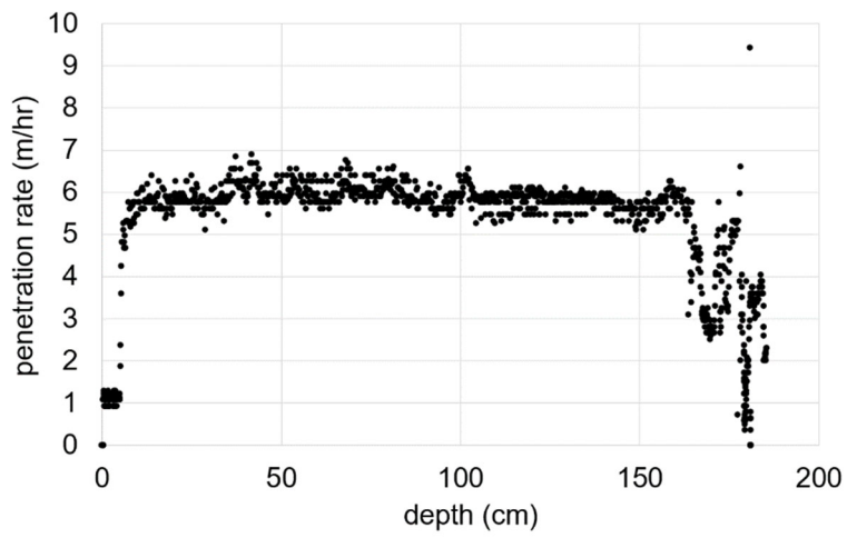
820 Figure 15-16 – Rate of penetration measured each second during a 45% power test in the artificial ice well at Jilin University. Aside from initialization and cessation effects, the rate of penetration showed little temporal variance during the steady drilling period ( 5.9 \pm 0.3 m/hr between 25 and 150 cm depth)
