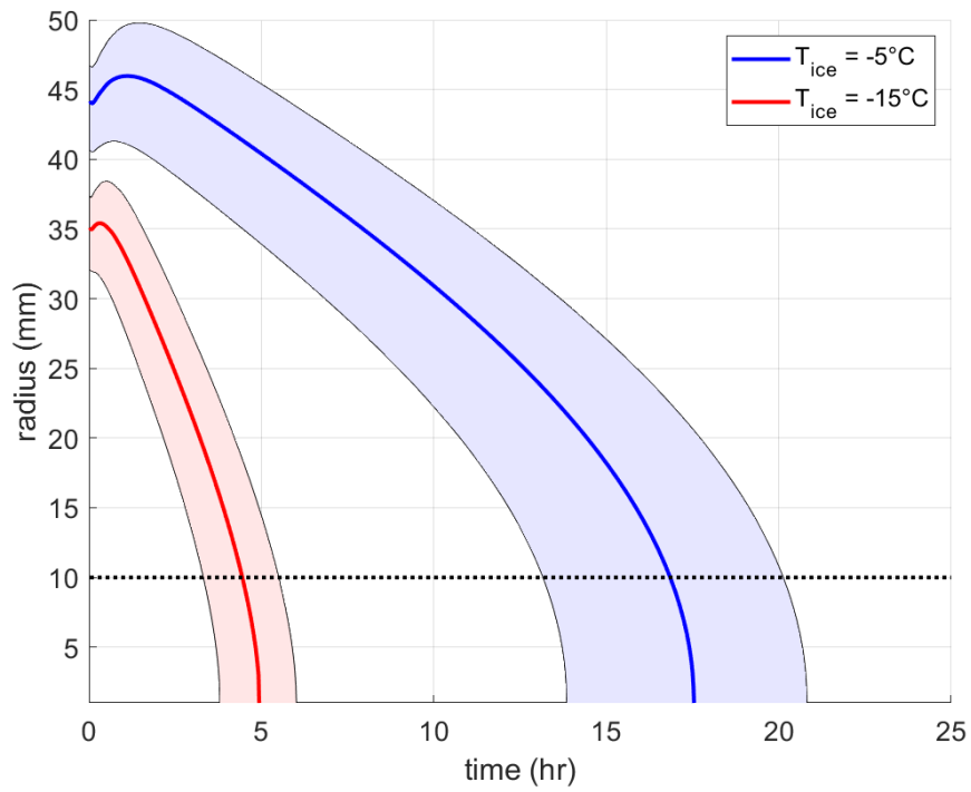
855 | Figure 22-23 – Borehole radius over time solved with a 1-D ice-water moving boundary heat diffusion model. These contrasting simulations depict the differing maximum borehole radii and decay timescales with ice temperatures of -5 and -15 °C. Shaded areas denote 75±25 °C uncertainty in initial borehole water temperature. Dotted line denotes a 10 mm radius equivalent to the effective cross-sectional area of the umbilical.
