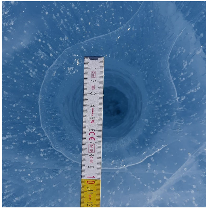
835 Figure 18-19 – Testing on the frozen Lake Tuto suggests that the effective borehole diameter of the melt tip is ~70 mm over a wide range of power levels and penetration rates.
