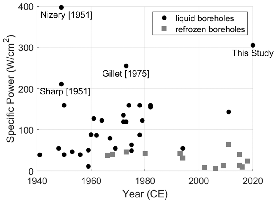
750 Figure 1 - Specific power of n = 46 electrothermal, or hot-point, drilling systems versus development year. Drilling systems are divided into those that operate in liquid and refrozen boreholes. Data compiled by Talalay [2019]. Four drilling systems of higher specific power ( > 200 \text{ W}/\text{cm}^2 ) are identified.
