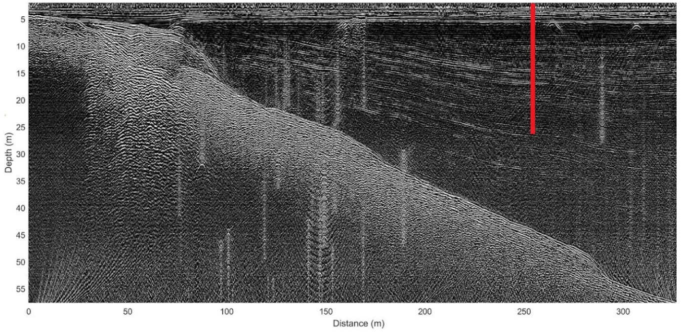
845 | Figure 20-21 – 100MHz ice-penetrating radar of ice thickness from the ice-sheet margin inland past the D-11 borehole (denoted in red) suggests an ice thickness of ~44 m at the D-11 drill site.
