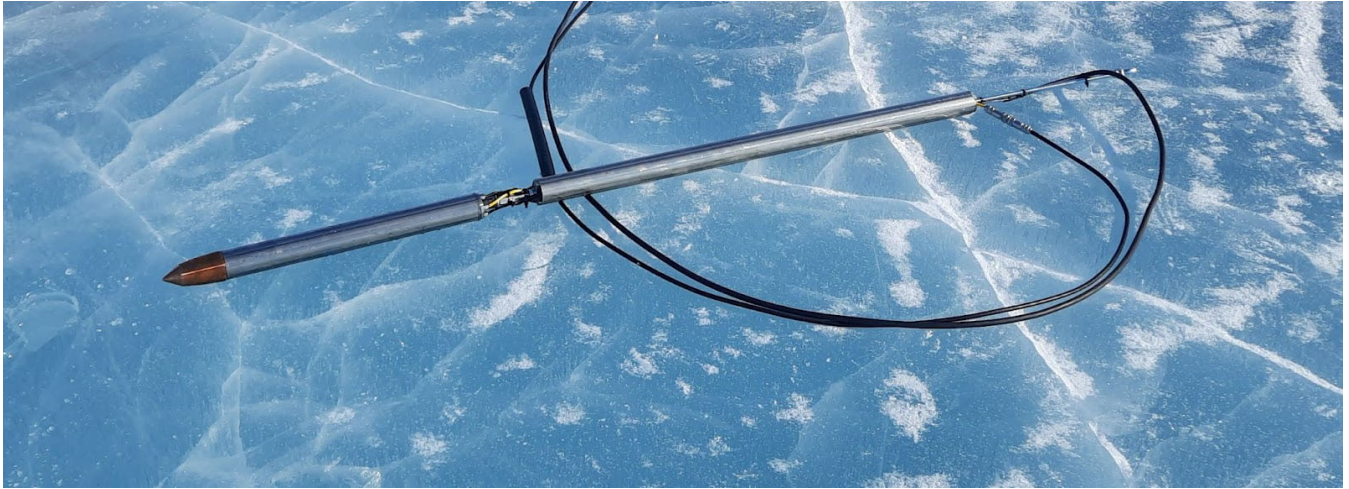
Figure 65 – Photo of a fully assembled v3 melt-tip on lake ice. The lower member (image left) is sealed and resin-filled while the upper member (image right) is unsealed and unfilled.
