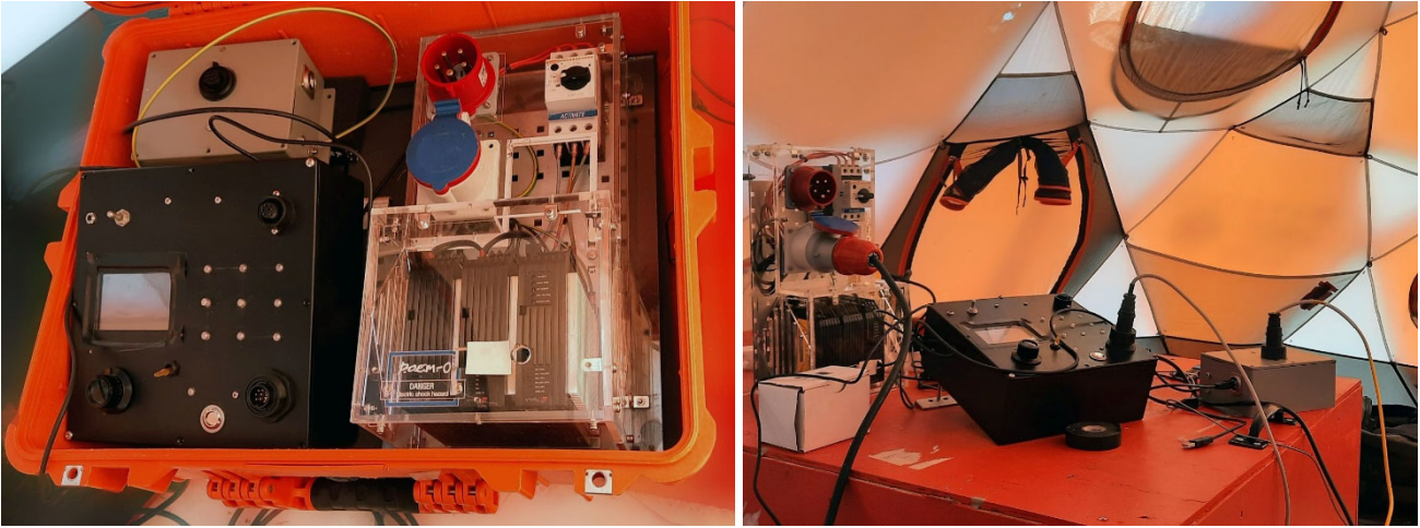
800 Figure 1244 – Interface connecting to the melt-tip, winch, and power supply at the ice-sheet testing site. Left: Interface elements transported inside a Pelican case. Right: Interface elements connected in the field tent.
