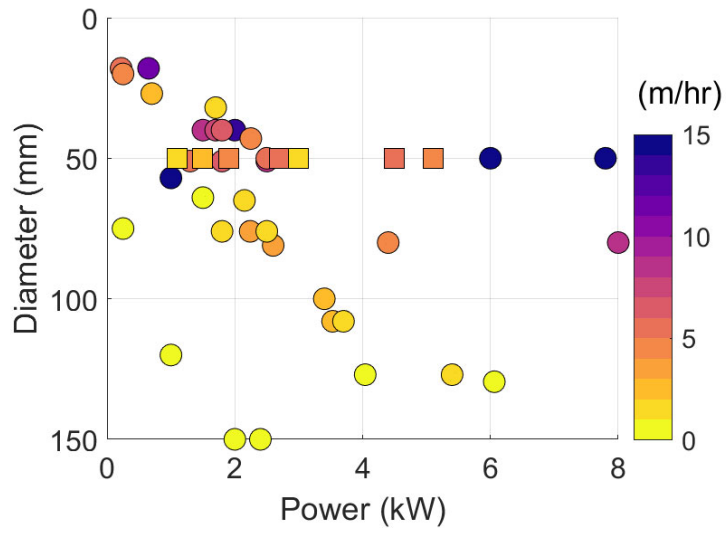
Figure 24-25 – Rate of penetration as dependent on melt-tip diameter and power. Circles denote previously described melt tip statistics compiled for n = 46 electrothermal ice drilling systems by Talalay [2019]. Squares denote our melt tip performance under both laboratory and field conditions described here.
