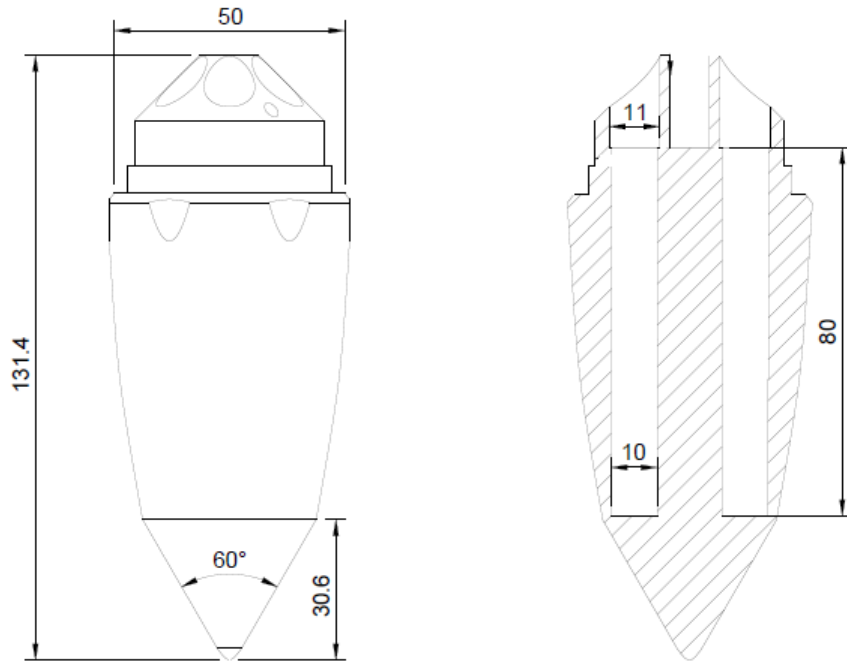
755 Figure 24 - Left: Technical drawing of the basic dimensions and sections of the melt tip. Right: Interior view of cartridge slots shows the depth placement of the 80 mm heated section of the cartridges.
