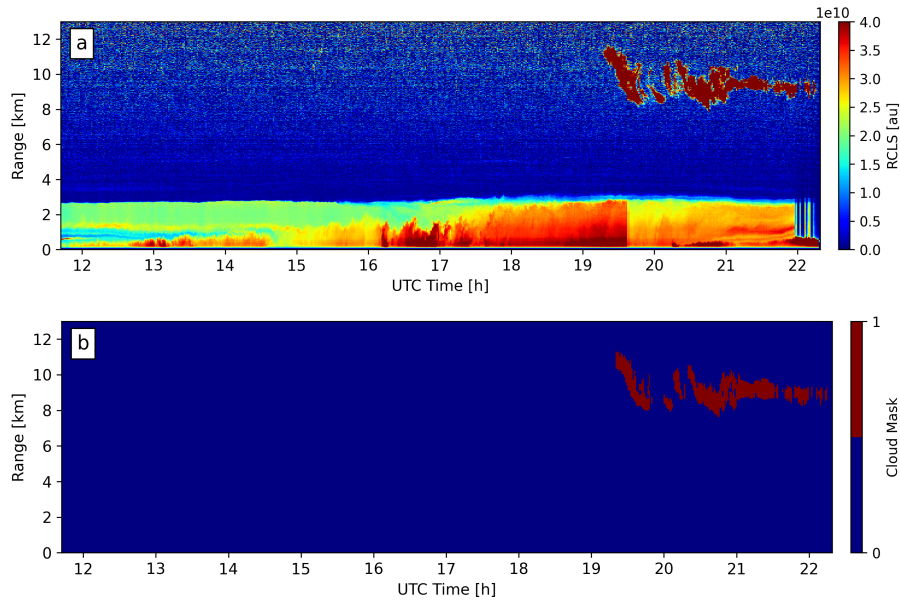
Figure 6. Level 1 data products showing the (a) RCLS and (b) cloud layer mask from measurements at layer mask for the Sao Paulo lidar station on 14 September 2020.
