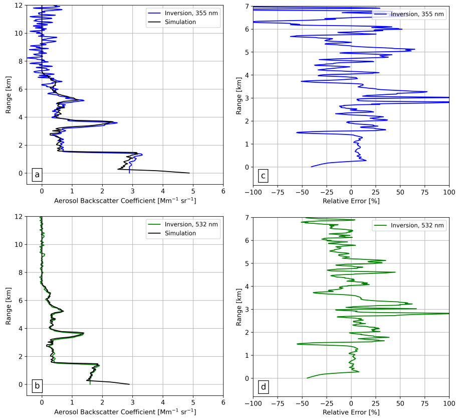
Figure 5. Left panels show a comparison of the aerosol backscatter coefficient ( \text{Mm}^{-1} \text{sr}^{-1} ) retrieved at (a) 355 nm (blue) and (b) 532 nm (green) with those used as input for the simulation (black lines). The right panels show the respective relative errors (%).
