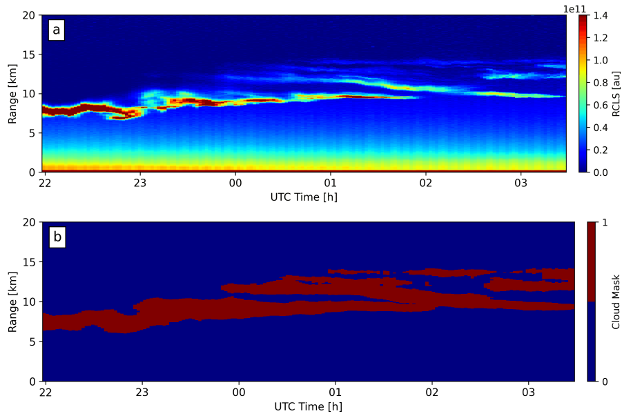
Figure 9. (a) RCLS (a) and layer-mask (b) from cloud layer mask for the Manaus lidar station from 22:00 UTC on 14 August 2011 to 3:30 UTC on 15 August 2011.
