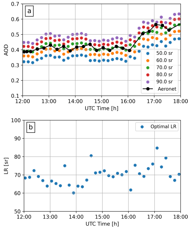
Figure 8. (a) AOD \tau_s at 532 nm measured by Aeronet (black) and obtained by the multi-LR lidar product and with using a set of predefined lidar ratios (colors) for the closest Aeronet value and Sao Paulo lidar station on 14 September 2020, from 12:00 to 18:00 UTC. (b) Optimal LRs values derived from each inversion.
