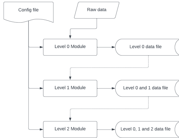
Figure 1. Flow diagram showing the structure of LPP version 1.1.0.2. Each module receives as input the data file produced as output in the previous module. A single configuration file is used for all the modules.
