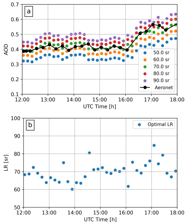
Figure 8. (a) AOD at 532 nm measured by Aeronet (black) and obtained by the multi-LR lidar product using a set of predefined lidar ratios (colors) for the Sao Paulo lidar station on 14 September 2020, from 12:00 to 18:00 UTC. (b) Optimal LR values derived from each inversion.
