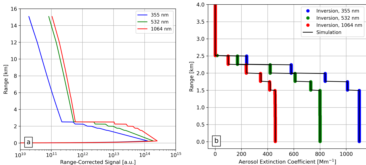
Figure 3. (a) Synthetic Range-corrected signals (a.u.) and (b) aerosol extinction coefficients ( \text{Mm}^{-1} ) retrieved with LPP (bullets) and used as input for the simulation (black lines) are shown for 355, 532 and 1064 nm.
