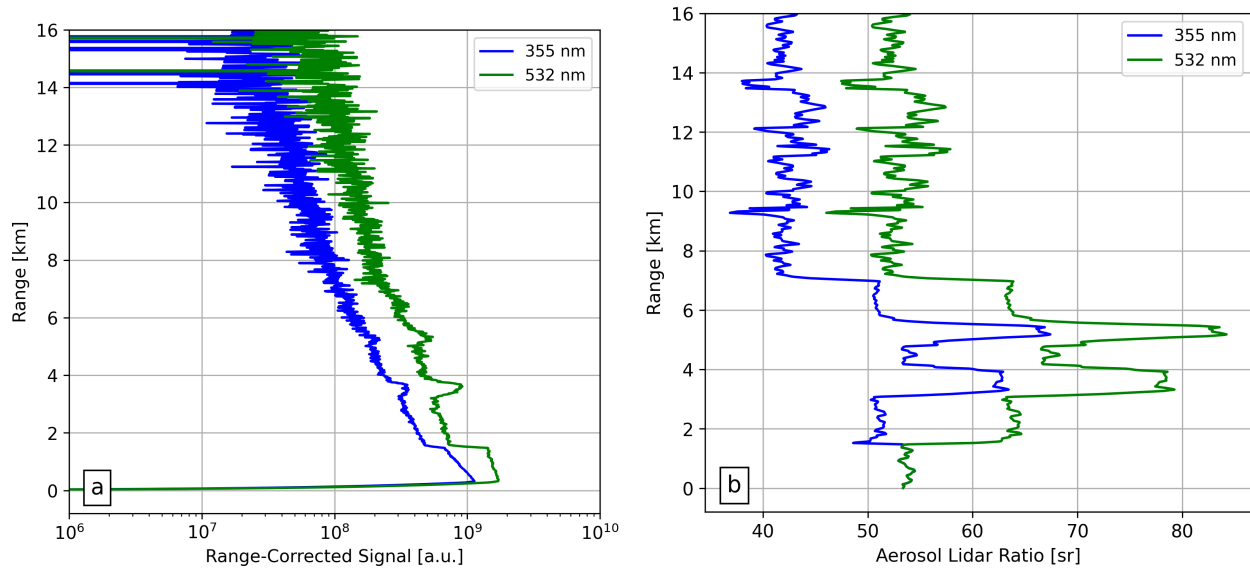
Figure 4. (a) Synthetic Range-corrected signals (a.u.) and (b) aerosol lidar ratio (sr) used as input for the simulation are shown for 355 nm and 532 nm. The retrievals shown in Fig. 5 assumed constant lidar ratios of 51 sr and 62 sr, respectively.
