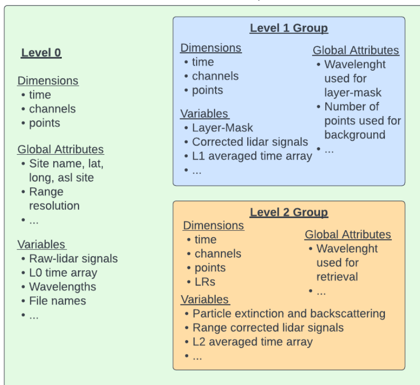
Figure 2. Schematic structure of the output files. Product data levels 1 and 2 are stored in subgroups named LX Data , while data level 0 data is stored in the file root tree. Dimensions and variables are explained in detail in the LPP's documentation on the GitHub repository (see section Open Science Development ).
