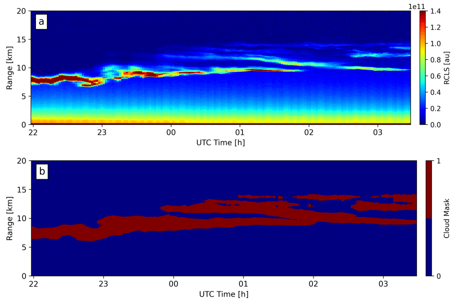
Figure 9. (a) RCLS and (b) cloud layer mask for the Manaus lidar station from 22:00 UTC on 14 August 2011 to 3:30 UTC on 15 August 2011.
