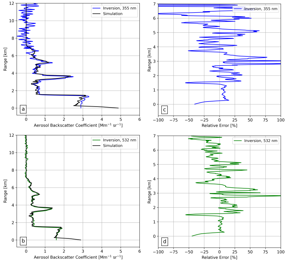
Figure 5. Left panels show a comparison of the aerosol backscatter coefficient ( \text{Mm}^{-1} \text{sr}^{-1} ) retrieved at (a) 355 nm and (b) 532 nm with those used as input for the simulation (black lines). The right panels show the respective relative errors (%).
