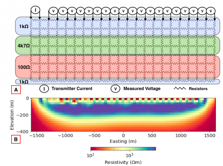
195 Figure 9: Simulated inversion for a dipole–dipole arrangement in the resistive layer model format (a) shows that the implementation of the measurement treatment can be performed by the equipment in loco with good performance, even though no configurations or adjustments were made to improve the results used for testing the programming and automation processes. In this validation test, we considered only three horizontal layers of the mesh of resistors with values of 1000 \Omega m, 4700 \Omega m, and 100 \Omega m. It is possible to identify clear features, such as the separation of layers (b), vertical discontinuity, 200 and order of magnitude of the resistivity, which are compatible with the values used in the test.
