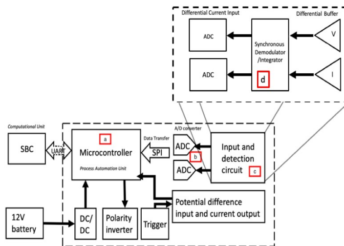
Figure 5: Schematic of the main circuit components developed for the prototype.
