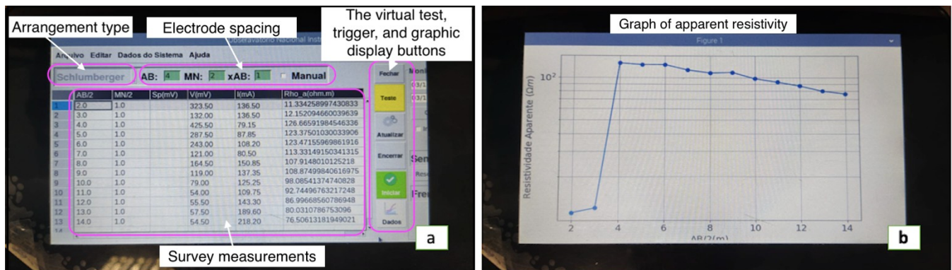
Figure 3: Computer unit running man-machine interface for georesistivity meter configuration demonstrating the capture of geoelectric data (a). Graphical implementation demonstration based on data obtained in a field survey, relating apparent resistivity \rho_a to AB/2 injection electrode openings (b).
