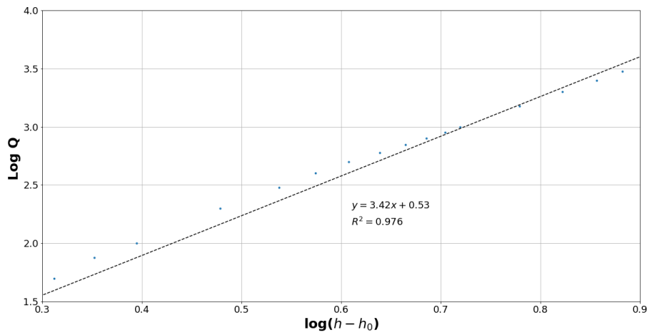
Figure 8 (Logarithm) Discharge vs stage relationship: combined roughness.
