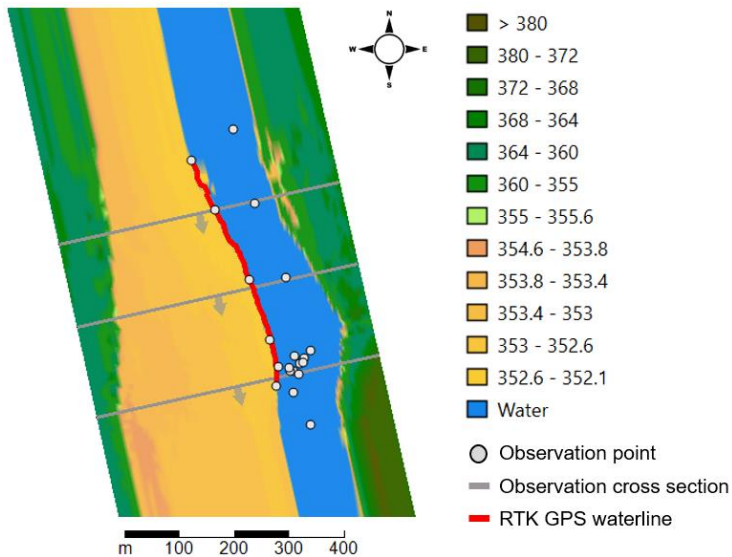
Figure 6 Visual representation of the discharge model at a discharge of 191 m 3 /s with n = 0.014 s/m 1/3
