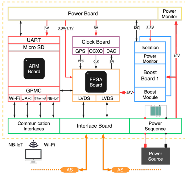
Figure 2: Hardware structure diagram of PSU.
