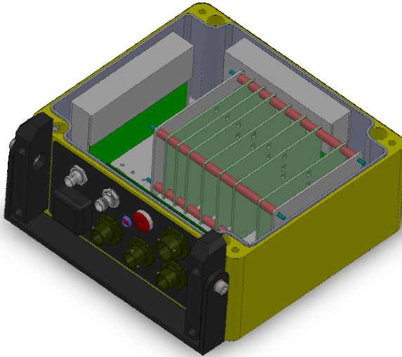
415 Figure 3: Three-dimensional structure diagram of PSU's external case.
