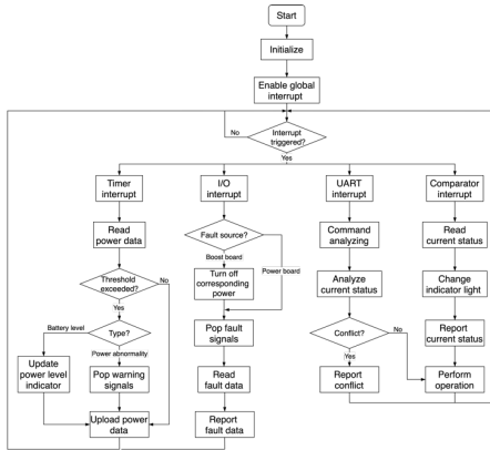
425 Figure 7: Power board software program flow chart
