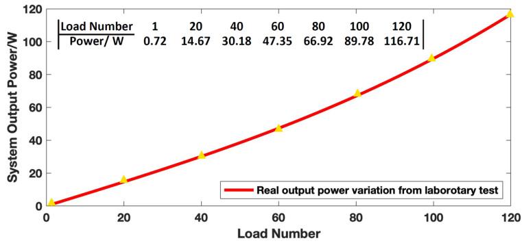
Figure 9: Output power evaluation test
