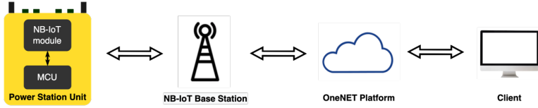
420 Figure 5: NB-LoT based networking topology
