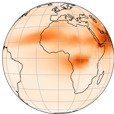
CAMS reanalysis AOD at 550 nm Jul-15
