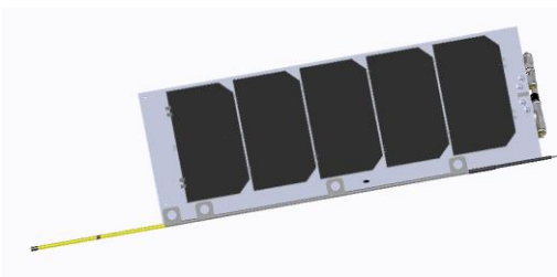
Figure 34. 40 mm long probe sticking out of a 40 mm long boom (both in yellow) at the extremity of the solar panel. Both the probe and the boom are 2 mm outer diameter gold coated Ti cylinders.
