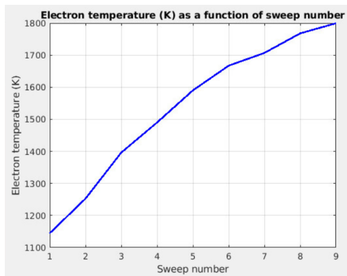
340 Fig. 4516. Electron temperature computed without taking into account the probe surface charging as a function of the sweep number for a series of 9 consecutive linear sweeps from -5 V to +13 V.
