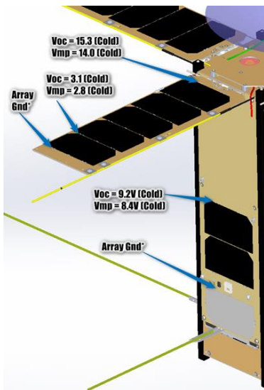
140 Figure 45. Location of the solar cells and interconnects on the solar panels (credit AAC Clyde Space AB).
