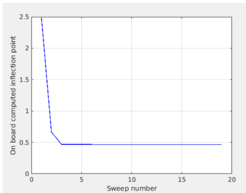
Figure 1412. Inflection point computed on board SLP after each sweep for a series of 19 consecutive nominal sweeps.
