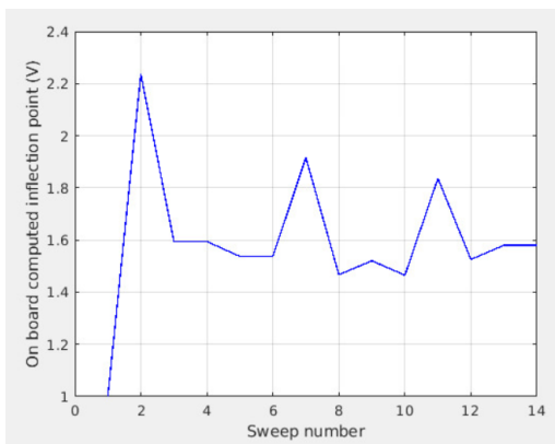
Figure 1314. Inflection point computed on board SLP after each sweep for a series of 14 consecutive sweeps with 60 bias steps. Data acquired in flight on 30.01.2021 from 13:03:53 to 13:04:06.
