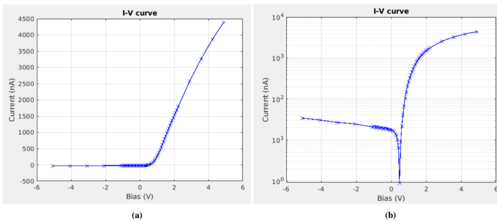
Figure 1313. In-flight measured I-V characteristic with 60 data points acquired on 30.01.2021 at 13:03:59 UTC. (a) linear scale, (b) semi-logarithmic scale.
