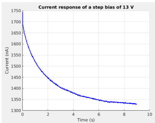
Fig. 1617. Current response to a 13 V bias.
