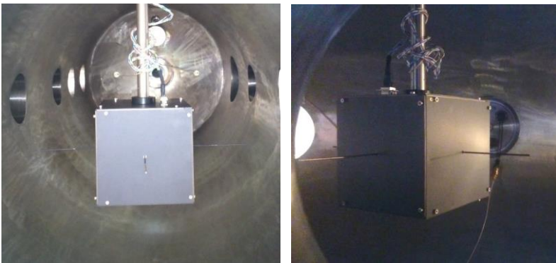
160 Figure 56. Picture of the electrically representative PICASSO mock-up in the plasma chamber.
