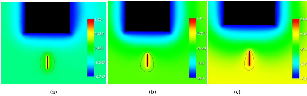
210 Figure 78. Plasma potential around the S/C mock-up when a bias of 2 V (a), 4.75 V (b) and 10.25 V (c) is applied on the probe, together with the iso level curve at 0.05V (linear scale, in V).
