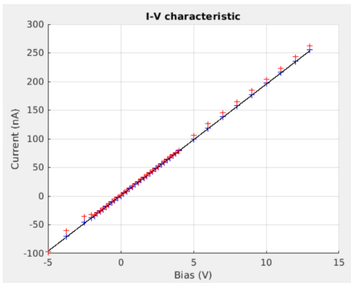
265 Figure 1011. Measured I-V characteristics when the probe is connected directly to a 50 Mohm resistor. Delay between samples set to 300 \mu s (red) and 600 \mu s (blue). For reference, the expected ideal curve is plotted in black.
