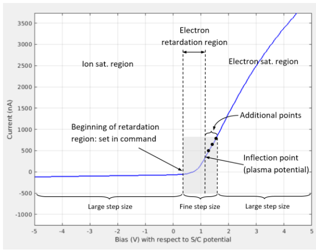
Figure 2. Example of sweep using the adaptive algorithm.
