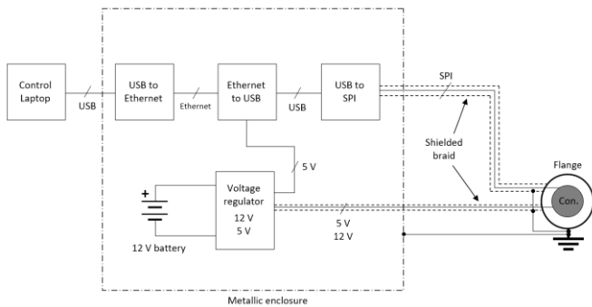
Figure 67. EGSE to test SLP and the PICASSO mock-up in the plasma chamber.
