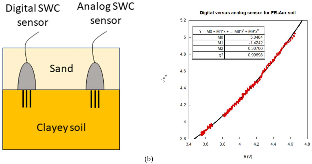
Figure 3. (a) Analog and digital FDR sensors cross-calibration configuration (b) Graphic comparison of the square root of the real part of relative dielectric permittivity, indicated by the digital FDR sensor, versus the SWC \theta value (in V) indicated by the analog FDR sensor. The table indicates the second-degree polynomial regression and the corresponding determination coefficient R^2 .
