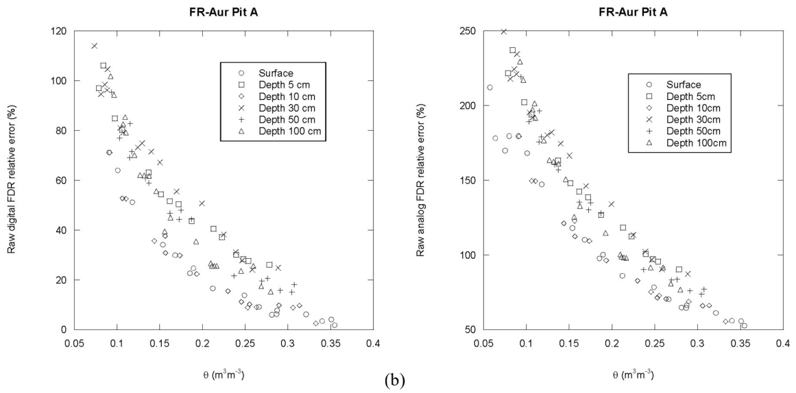
280 Figure 6. Relative error of SWC estimated (a) with a factory-calibrated digital sensor based on the real part of the dielectric permittivity or (b) with a factory-calibrated analog sensor based on the modulus of the dielectric permittivity, versus real SWC into pit A at six depths.
