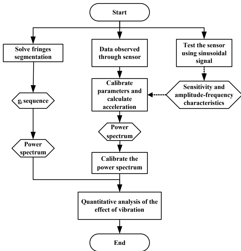
150 Figure 7: Data processing flow
