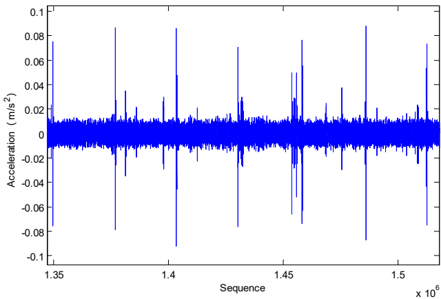
Figure 11: Vibration acceleration data
