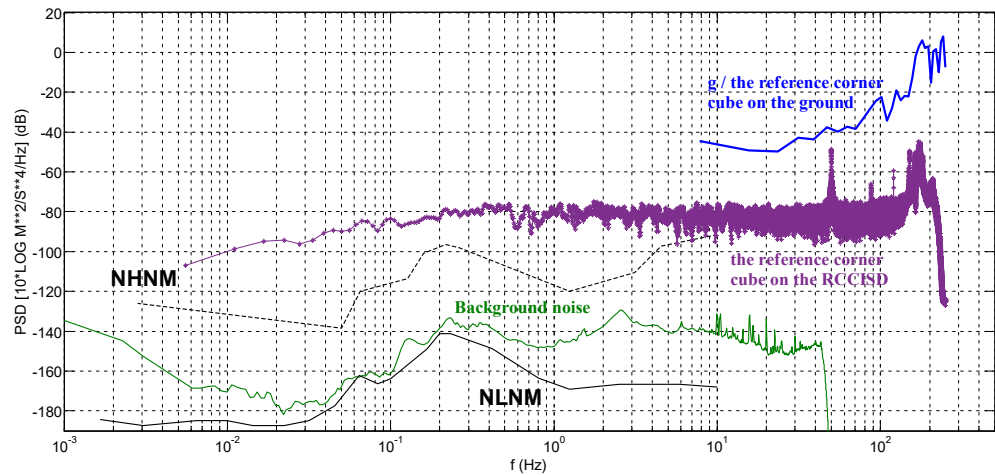
Figure 15:The PSD of experimental data
