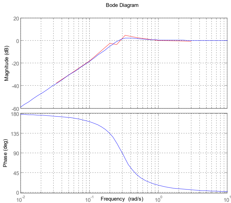
Figure 9: Calibrated transfer function
