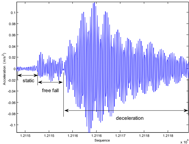
200 Figure 12.:Vibration data during a free fall
