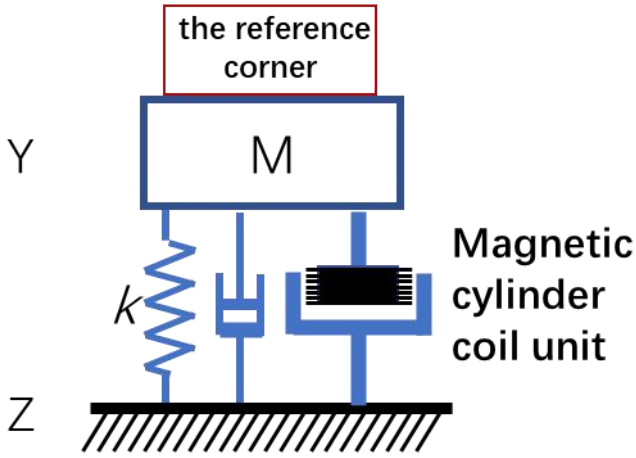
Figure 3: Principle model
