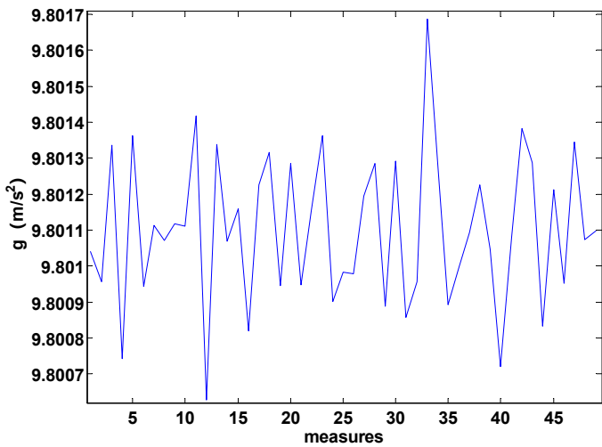
Figure 13: The sequence of absolute gravitational acceleration
