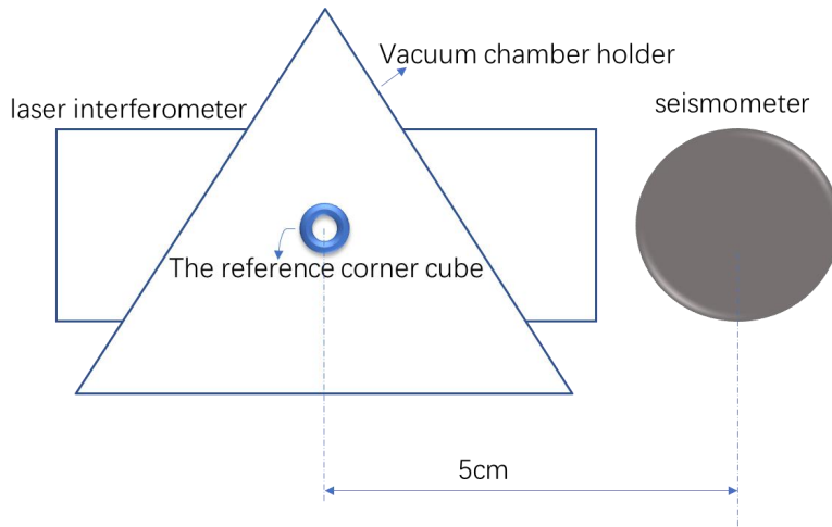
Figure 2: Schematic diagram of synchronous observation position of seismograph
