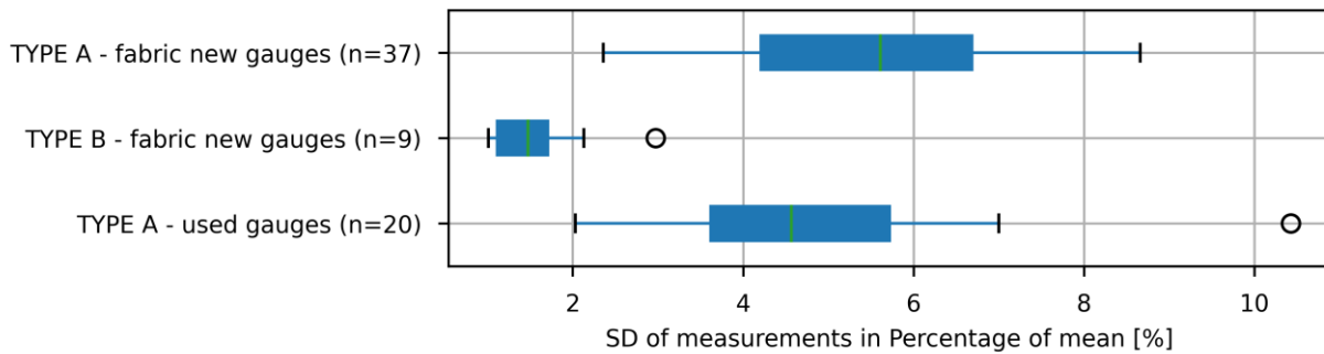
Figure 5: Comparison between used and fabric new gauges – SD of single measurements in percentage of mean
