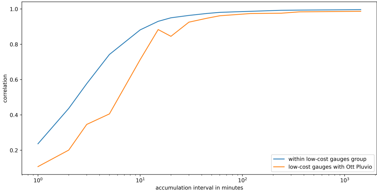
Figure 11: Average Correlation values for different accumulation intervals (low-cost vs low-cost and low-cost vs Ott Pluvio)
