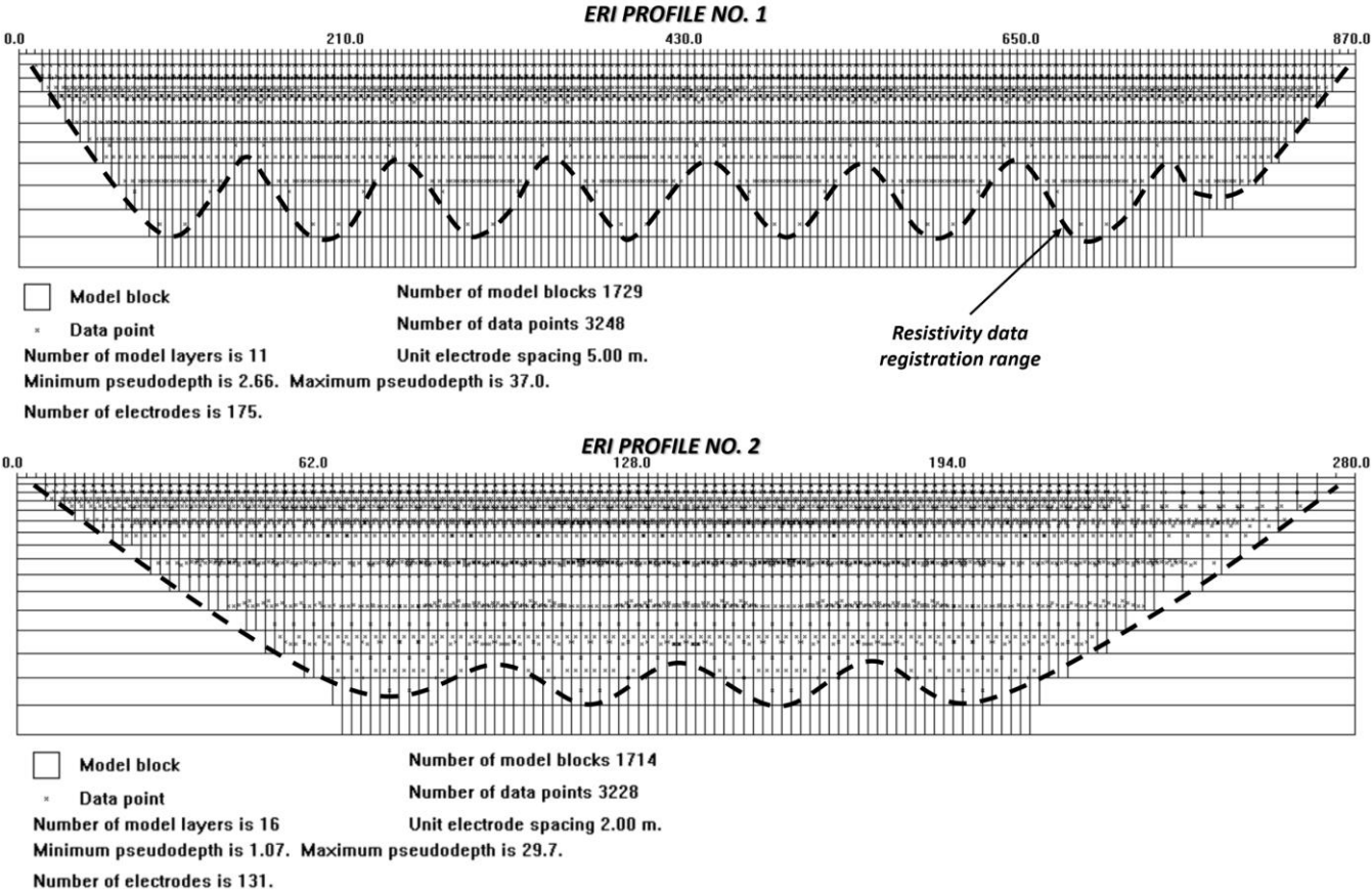
Figure 5: Electrical resistivity data points distribution and arrangement of model blocks: ERI profile No. 1 and 2 at the Rospuda site
