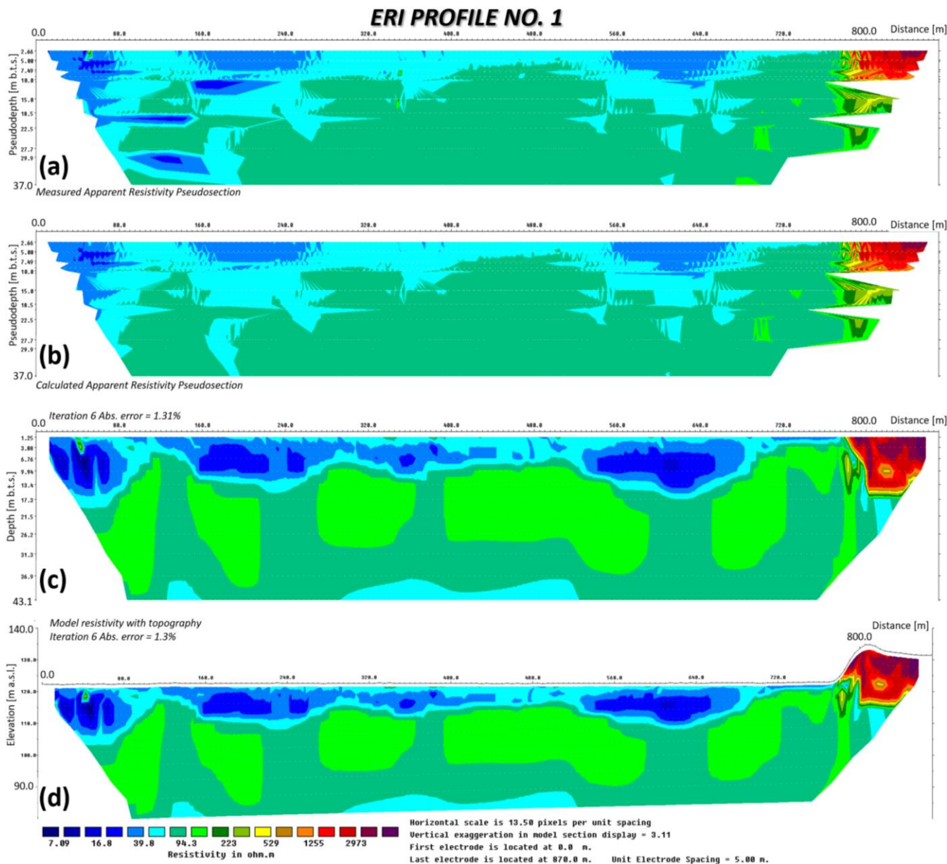
Figure 6: ERI profile No. 1 at the Rospuda site: (a) apparent resistivity data, (b) calculated apparent resistivity data, (c) inverted resistivity model, and (d) inverted resistivity model with topography.
