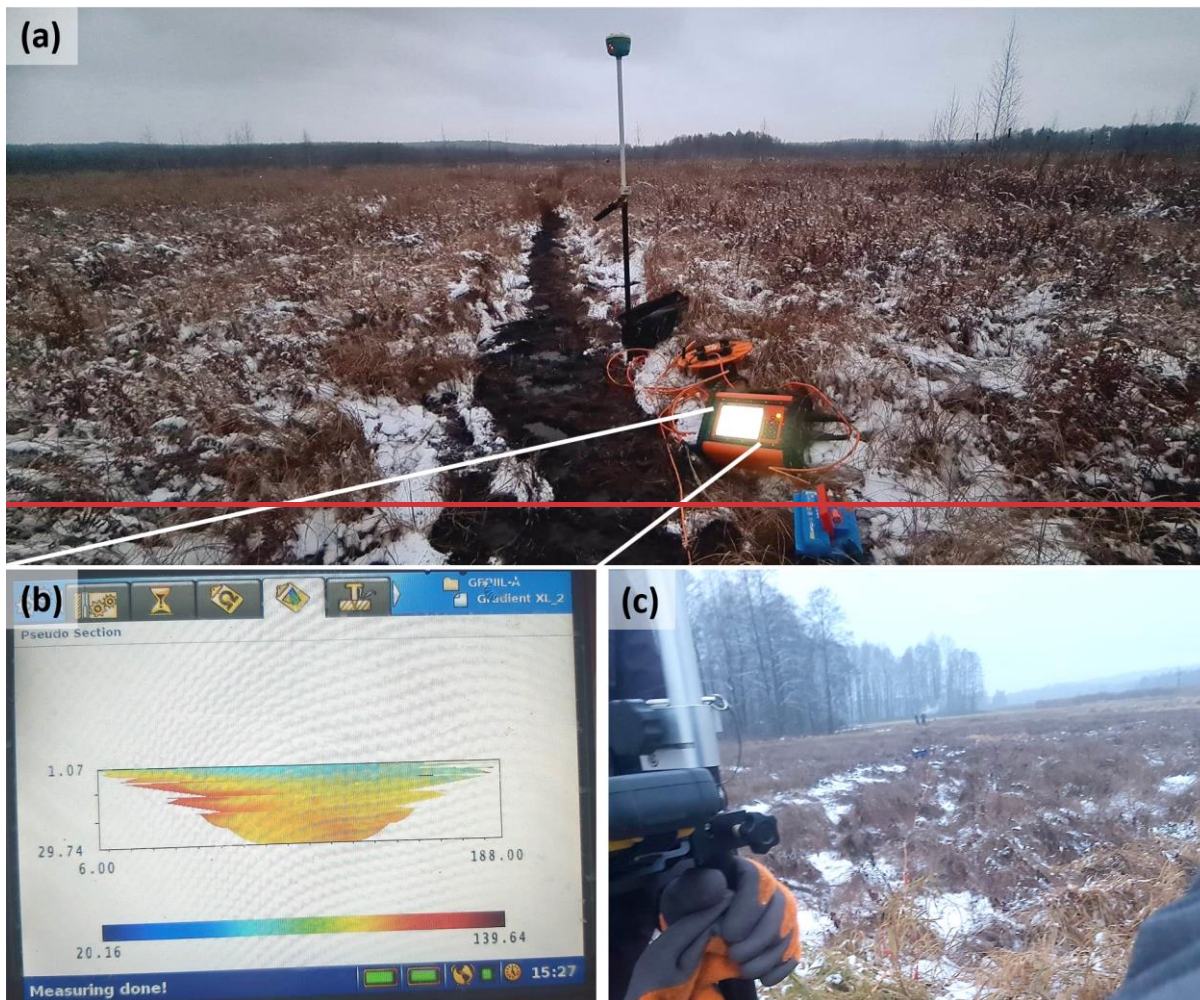
Figure 3: Acquiring ERI field data with multi-electrode (a) 12-point light Abem Terrameter LS-2 set-up at ERI profile No. 1, (b) raw visualization of results; (c) ERI profile No. 2.
