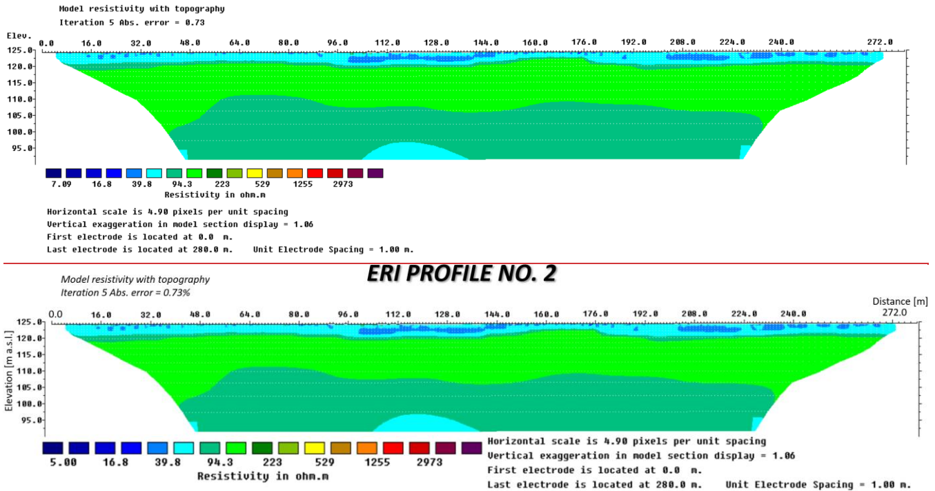
155 Figure 7: ERI profile No. 2 at the Rospuda site - inverted resistivity model with topography.
