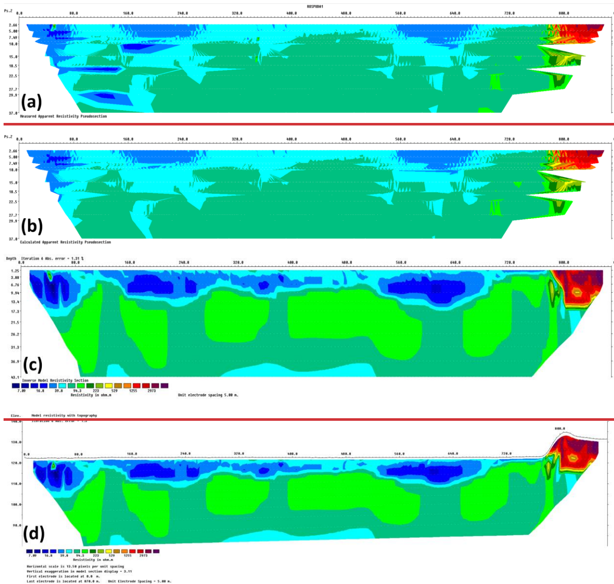
Figure 5: ERI profile No. 1 at the Rospuda site: (a) apparent resistivity data, (b) calculated apparent resistivity data, (c) inverted resistivity model, and (d) inverted resistivity model with topography.
