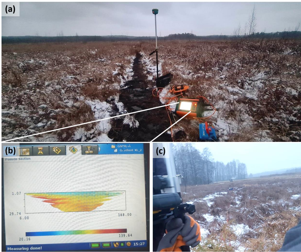
Figure 4: Acquiring ERI field data with multi-electrode (a) 12-point light Abem Terrameter LS-2 set-up at ERI profile No. 1, (b) raw visualization of results; (c) ERI profile No. 2.
