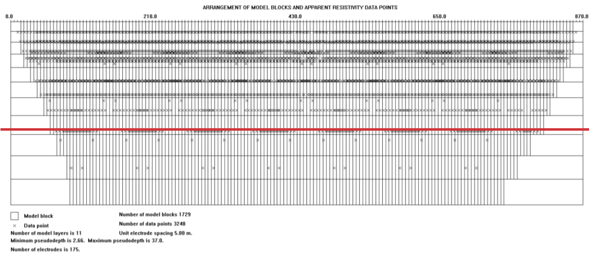
Figure 4: ERI profile No. 2 at the Rospuda site: the electrical resistivity data points distribution.
