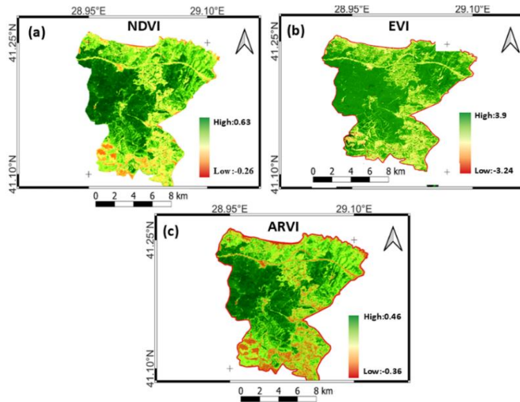
Figure 4. Calculated from Sentinel-2 images with plugins (a) NDVI indices, (b) EVI indices, and (c) ARVI indices.
